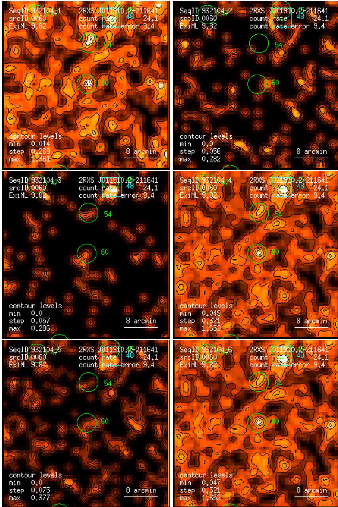
Figure 60: RASS 932104: detection 0060: band rate images, Gaussian filter: (1) PSPC channels 11 – 41, (2) 52 – 90, (3) 91 – 201, (4) 11 – 235, (5) 52 – 201, (6) 11 – 201. Broad band rates in counts/ks. Band rate contour levels in counts/ks/arcmin 2 .
