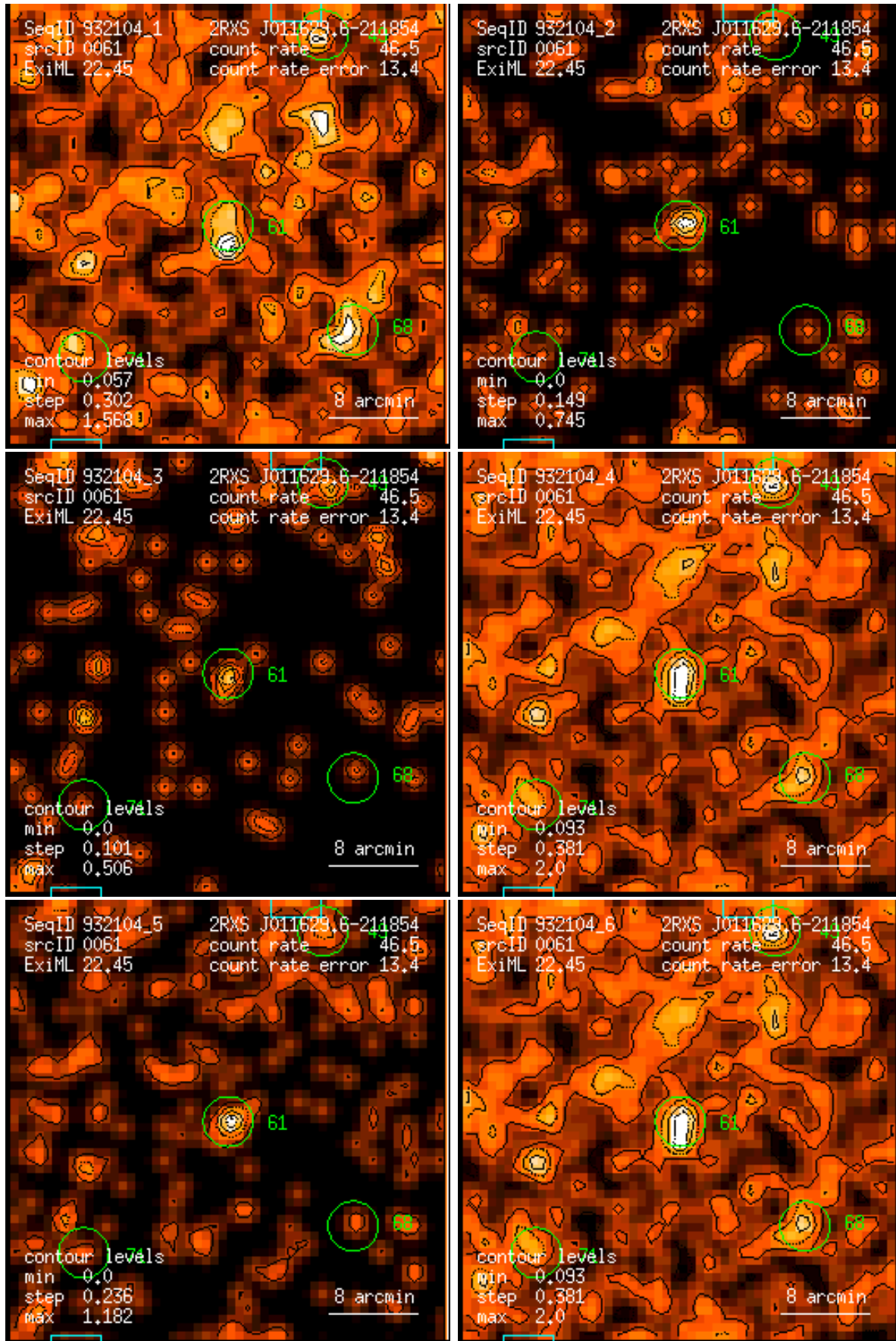
Figure 61: RASS 932104: detection 0061: band rate images, Gaussian filter: (1) PSPC channels 11 – 41, (2) 52 – 90, (3) 91 – 201, (4) 11 – 235, (5) 52 – 201, (6) 11 – 201. Broad band rates in counts/ks. Band rate contour levels in counts/ks/arcmin 2 .
