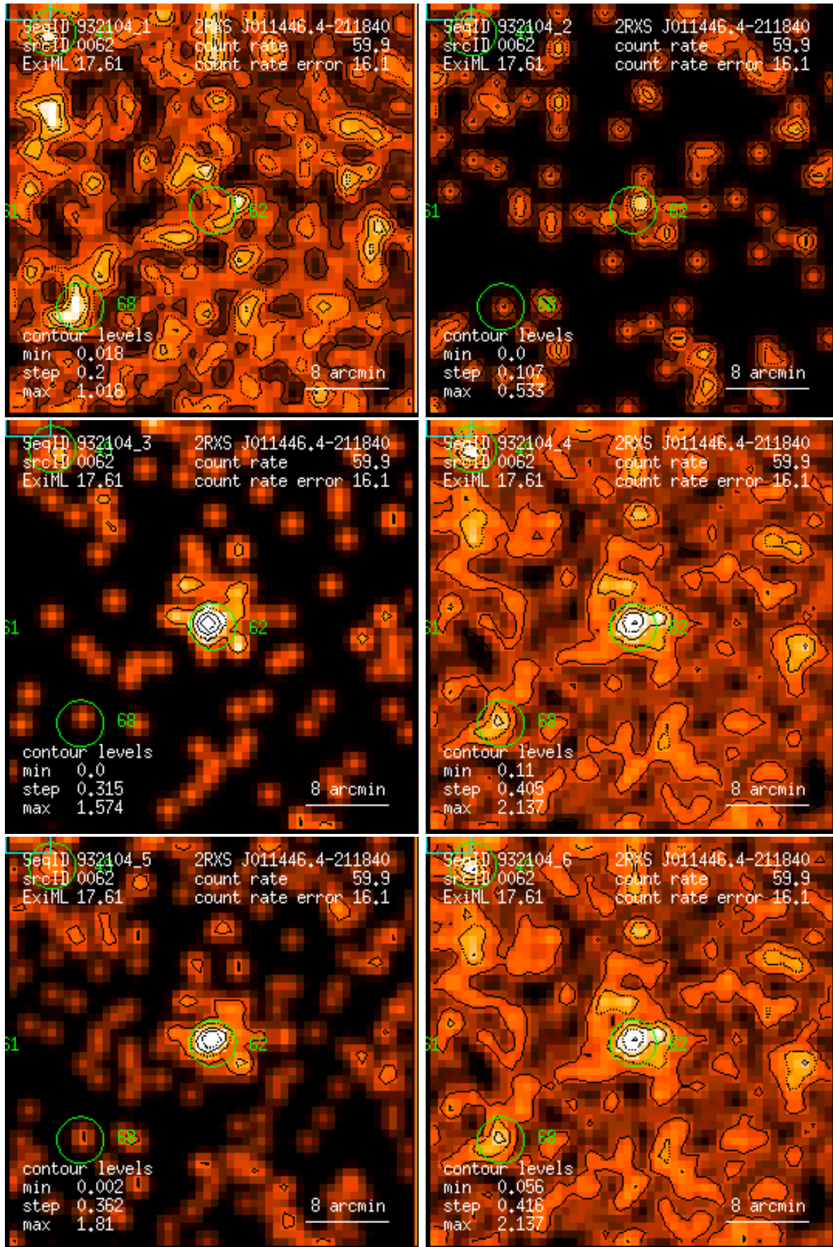
Figure 62: RASS 932104: detection 0062: band rate images, Gaussian filter: (1) PSPC channels 11 – 41, (2) 52 – 90, (3) 91 – 201, (4) 11 – 235, (5) 52 – 201, (6) 11 – 201. Broad band rates in counts/ks. Band rate contour levels in counts/ks/arcmin 2 .
