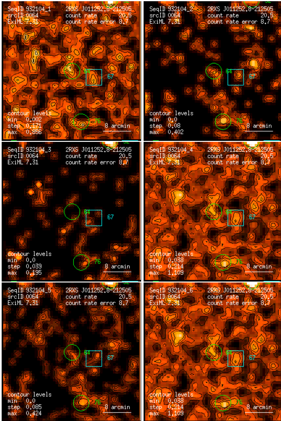
Figure 64: RASS 932104: detection 0064: band rate images, Gaussian filter: (1) PSPC channels 11 – 41, (2) 52 – 90, (3) 91 – 201, (4) 11 – 235, (5) 52 – 201, (6) 11 – 201. Broad band rates in counts/ks. Band rate contour levels in counts/ks/arcmin 2 .
