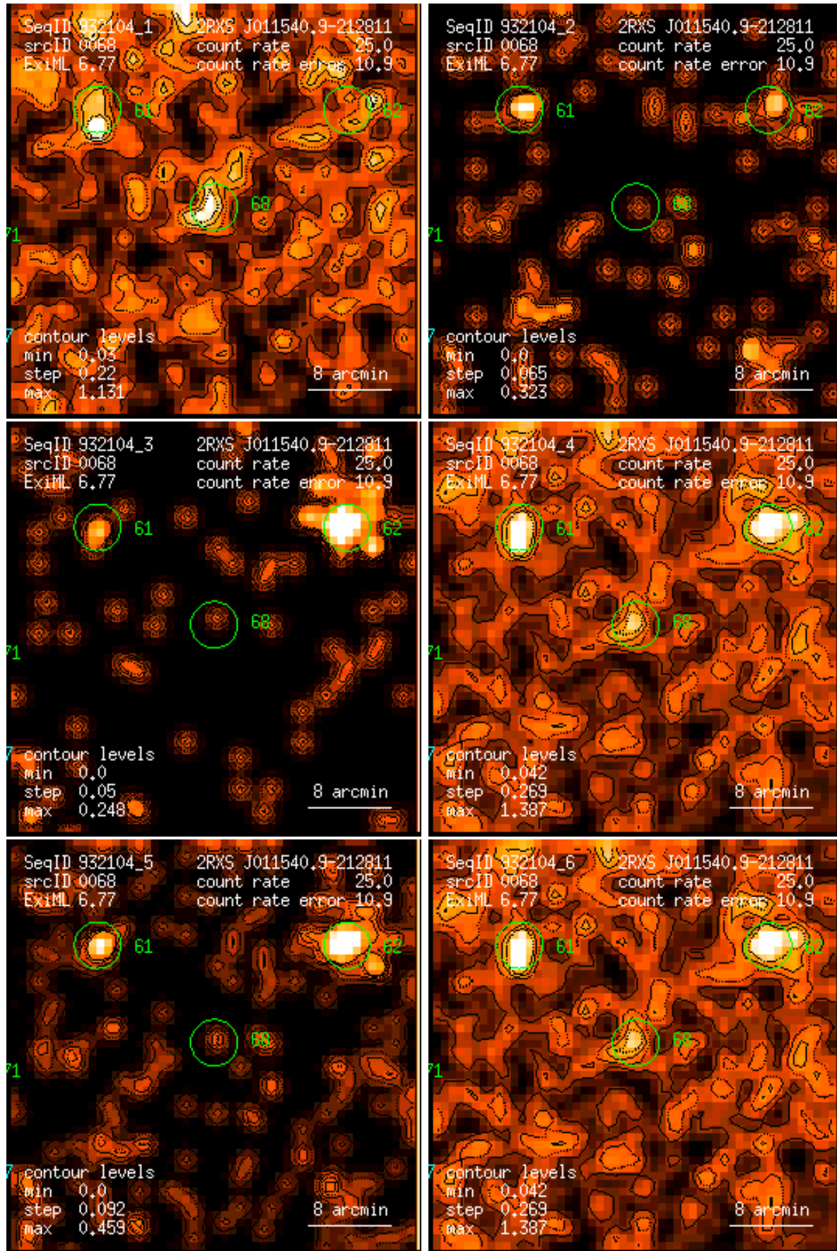
Figure 68: RASS 932104: detection 0068: band rate images, Gaussian filter: (1) PSPC channels 11 – 41, (2) 52 – 90, (3) 91 – 201, (4) 11 – 235, (5) 52 – 201, (6) 11 – 201. Broad band rates in counts/ks. Band rate contour levels in counts/ks/arcmin 2 .
