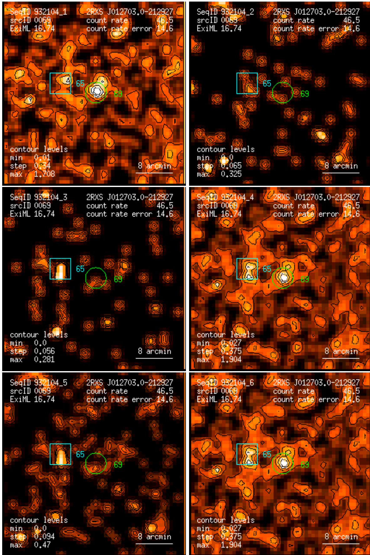
Figure 69: RASS 932104: detection 0069: band rate images, Gaussian filter: (1) PSPC channels 11 – 41, (2) 52 – 90, (3) 91 – 201, (4) 11 – 235, (5) 52 – 201, (6) 11 – 201. Broad band rates in counts/ks. Band rate contour levels in counts/ks/arcmin 2 .
