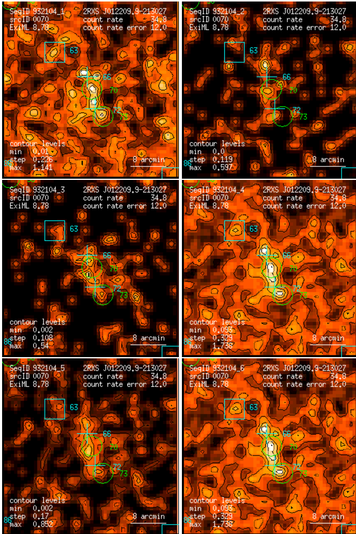
Figure 70: RASS 932104: detection 0070: band rate images, Gaussian filter: (1) PSPC channels 11 – 41, (2) 52 – 90, (3) 91 – 201, (4) 11 – 235, (5) 52 – 201, (6) 11 – 201. Broad band rates in counts/ks. Band rate contour levels in counts/ks/arcmin 2 .
