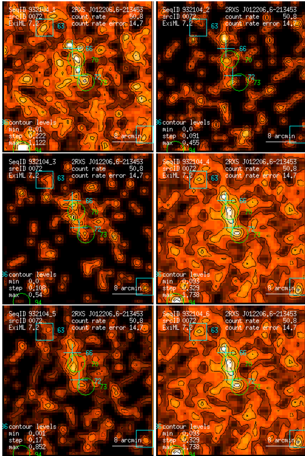
Figure 72: RASS 932104: detection 0072: band rate images, Gaussian filter: (1) PSPC channels 11 – 41, (2) 52 – 90, (3) 91 – 201, (4) 11 – 235, (5) 52 – 201, (6) 11 – 201. Broad band rates in counts/ks. Band rate contour levels in counts/ks/arcmin 2 .
