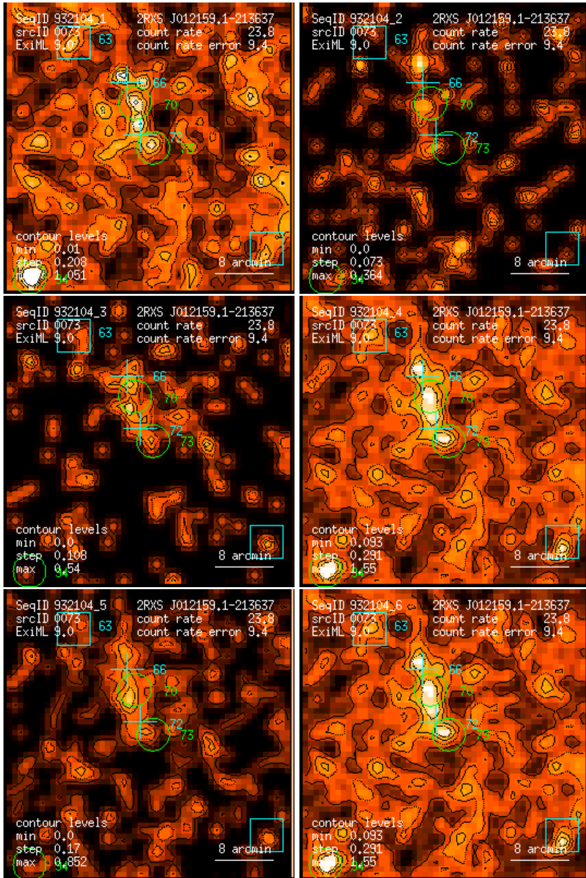
Figure 73: RASS 932104: detection 0073: band rate images, Gaussian filter: (1) PSPC channels 11 – 41, (2) 52 – 90, (3) 91 – 201, (4) 11 – 235, (5) 52 – 201, (6) 11 – 201. Broad band rates in counts/ks. Band rate contour levels in counts/ks/arcmin 2 .
