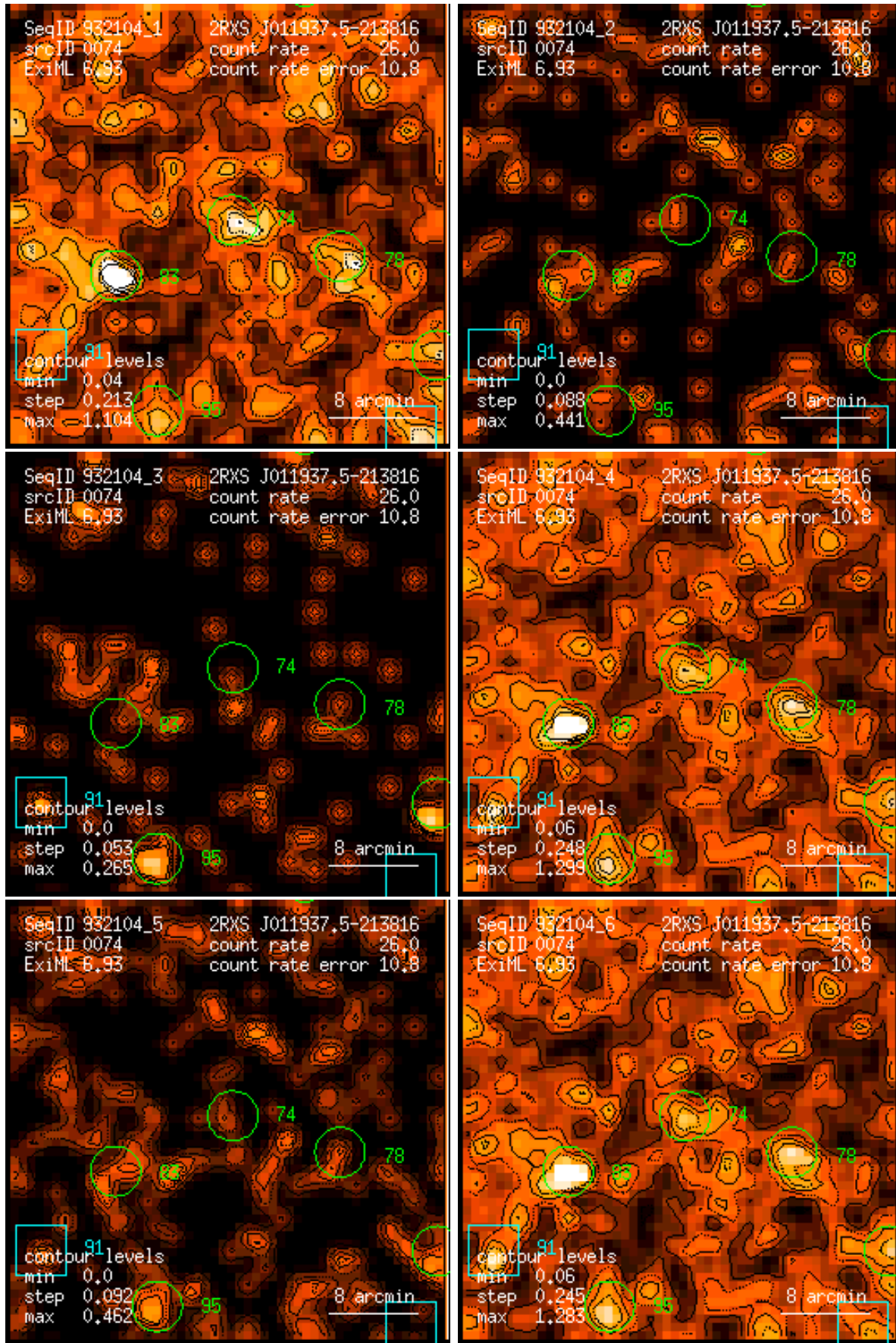
Figure 74: RASS 932104: detection 0074: band rate images, Gaussian filter: (1) PSPC channels 11 – 41, (2) 52 – 90, (3) 91 – 201, (4) 11 – 235, (5) 52 – 201, (6) 11 – 201. Broad band rates in counts/ks. Band rate contour levels in counts/ks/arcmin 2 .
