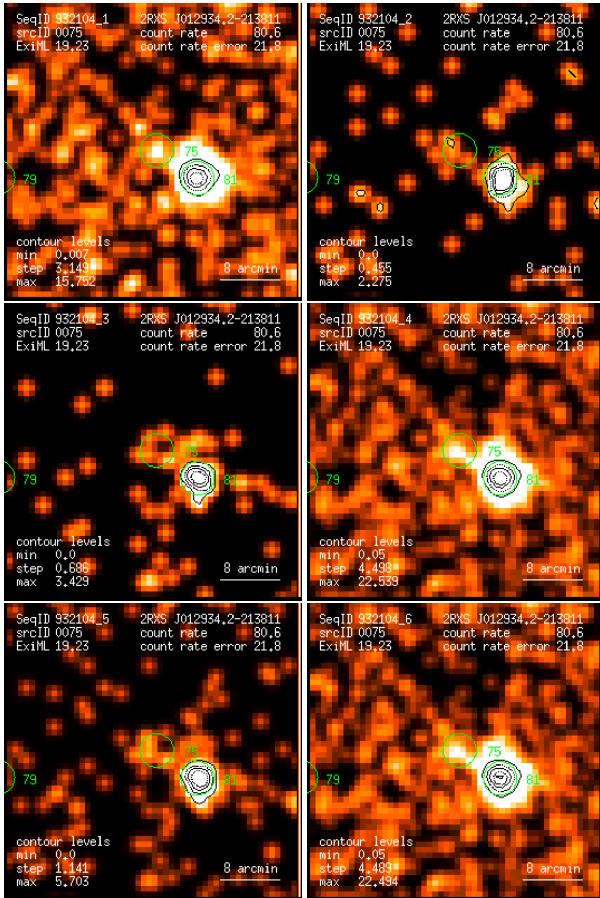
Figure 75: RASS 932104: detection 0075: band rate images, Gaussian filter: (1) PSPC channels 11 – 41, (2) 52 – 90, (3) 91 – 201, (4) 11 – 235, (5) 52 – 201, (6) 11 – 201. Broad band rates in counts/ks. Band rate contour levels in counts/ks/arcmin 2 .
