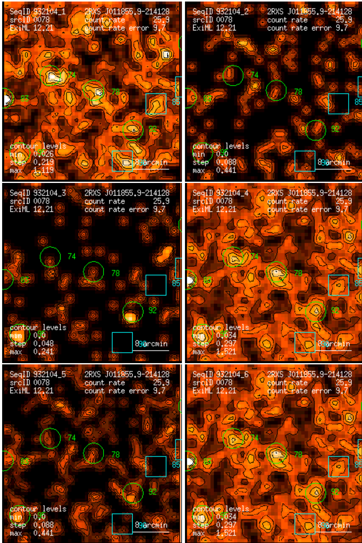
Figure 78: RASS 932104: detection 0078: band rate images, Gaussian filter: (1) PSPC channels 11 – 41, (2) 52 – 90, (3) 91 – 201, (4) 11 – 235, (5) 52 – 201, (6) 11 – 201. Broad band rates in counts/ks. Band rate contour levels in counts/ks/arcmin 2 .
