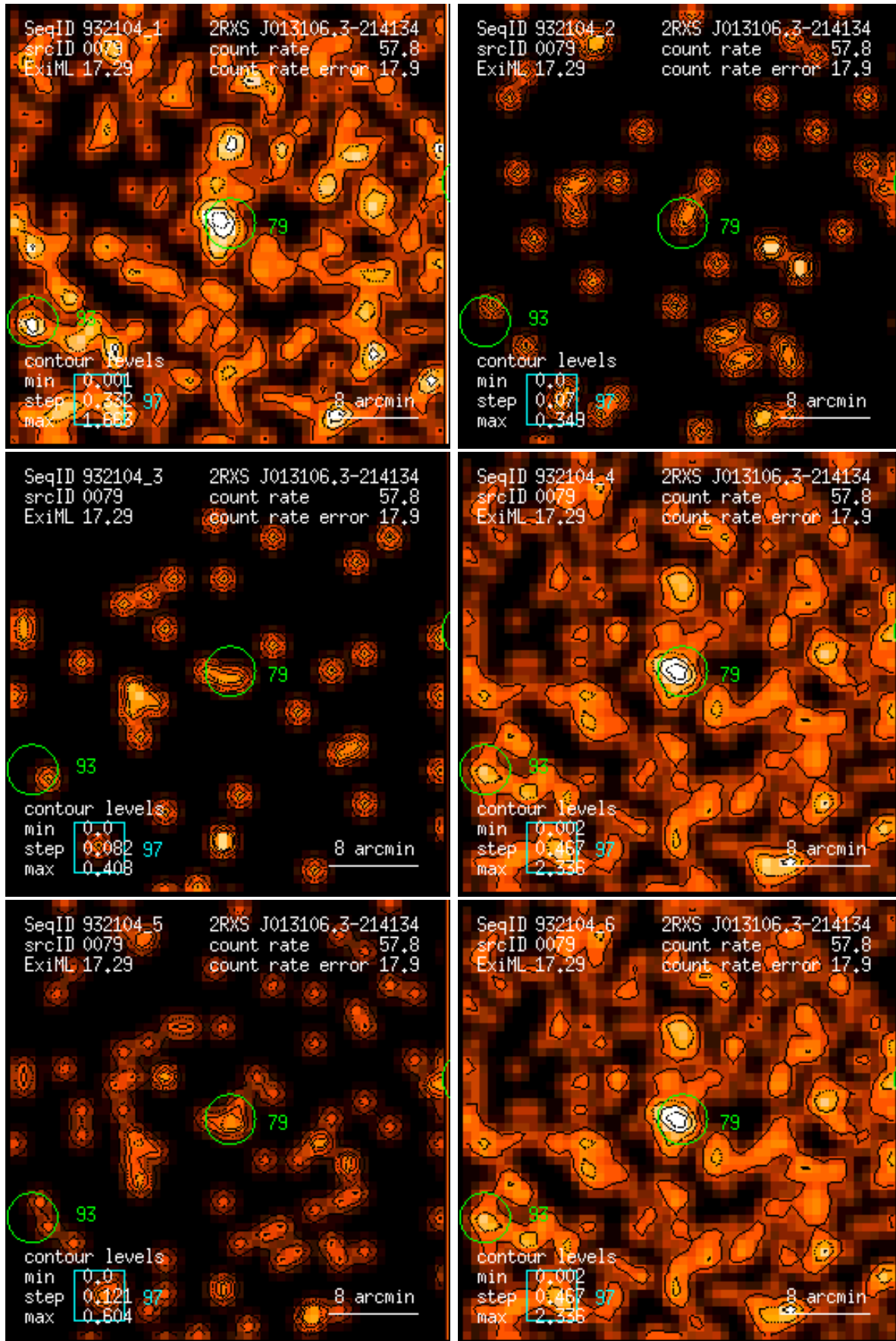
Figure 79: RASS 932104: detection 0079: band rate images, Gaussian filter: (1) PSPC channels 11 – 41, (2) 52 – 90, (3) 91 – 201, (4) 11 – 235, (5) 52 – 201, (6) 11 – 201. Broad band rates in counts/ks. Band rate contour levels in counts/ks/arcmin 2 .
