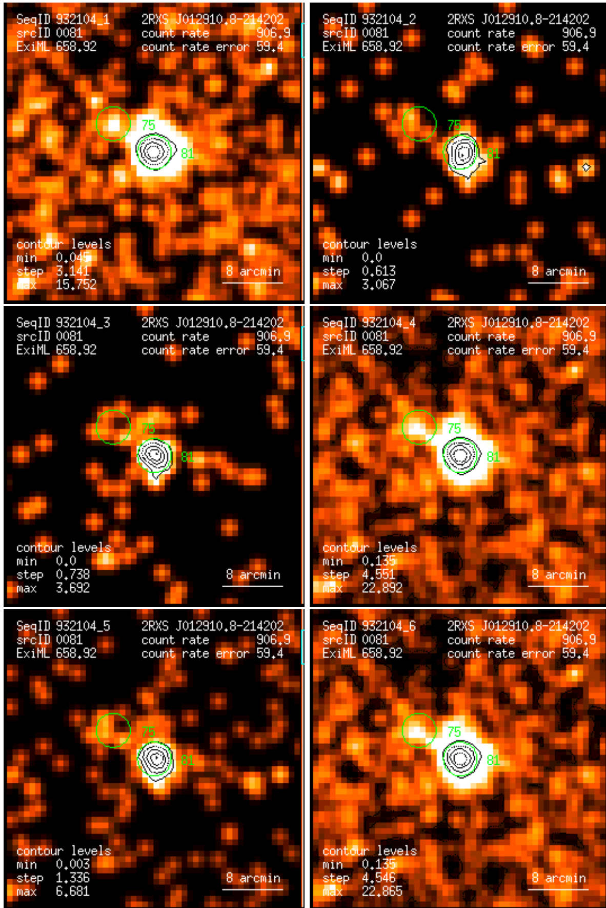
Figure 81: RASS 932104: detection 0081: band rate images, Gaussian filter: (1) PSPC channels 11 – 41, (2) 52 – 90, (3) 91 – 201, (4) 11 – 235, (5) 52 – 201, (6) 11 – 201. Broad band rates in counts/ks. Band rate contour levels in counts/ks/arcmin 2 .
