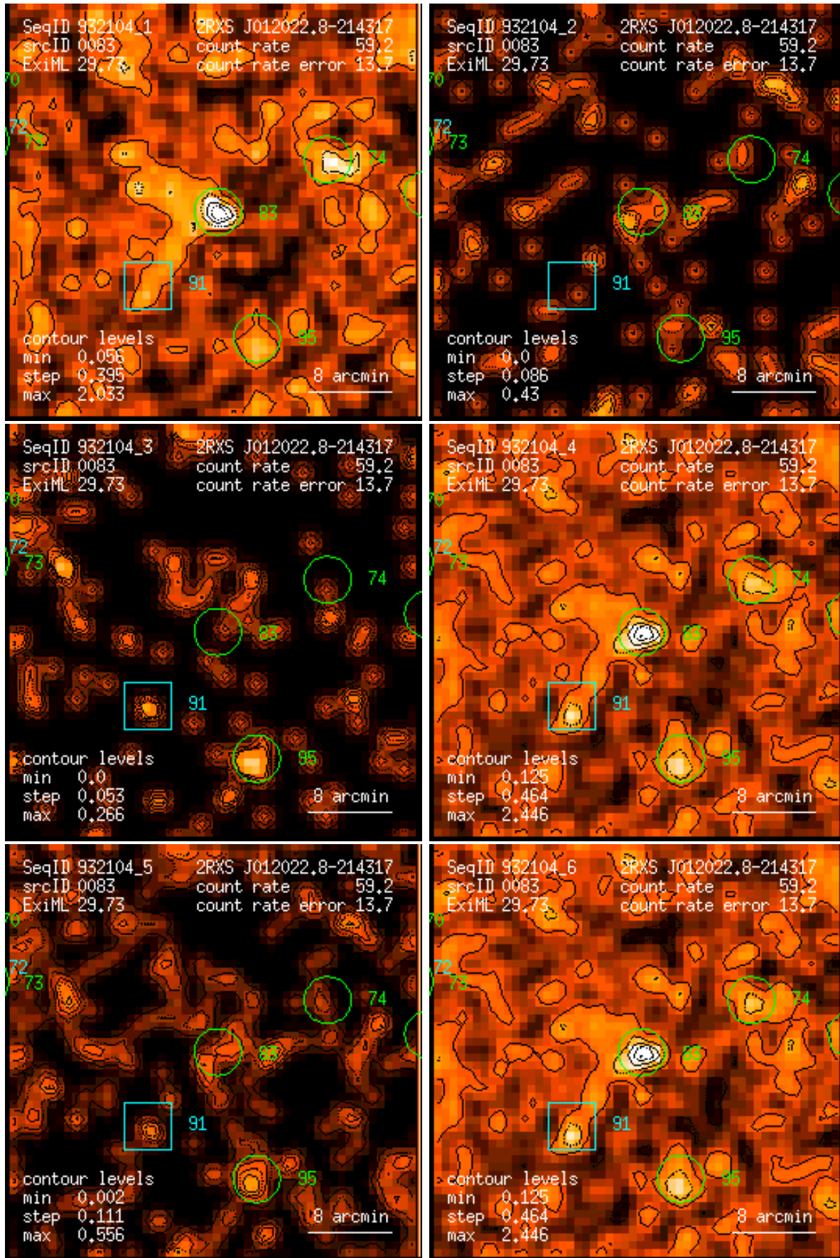
Figure 83: RASS 932104: detection 0083: band rate images, Gaussian filter: (1) PSPC channels 11 – 41, (2) 52 – 90, (3) 91 – 201, (4) 11 – 235, (5) 52 – 201, (6) 11 – 201. Broad band rates in counts/ks. Band rate contour levels in counts/ks/arcmin 2 .
