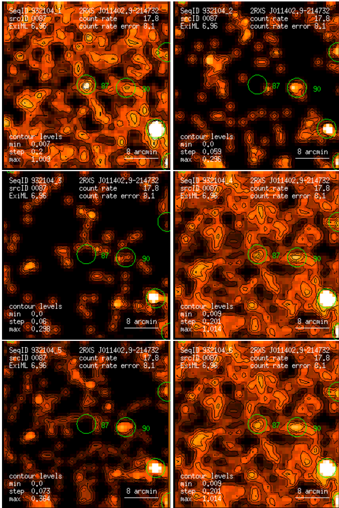
Figure 87: RASS 932104: detection 0087: band rate images, Gaussian filter: (1) PSPC channels 11 – 41, (2) 52 – 90, (3) 91 – 201, (4) 11 – 235, (5) 52 – 201, (6) 11 – 201. Broad band rates in counts/ks. Band rate contour levels in counts/ks/arcmin 2 .
