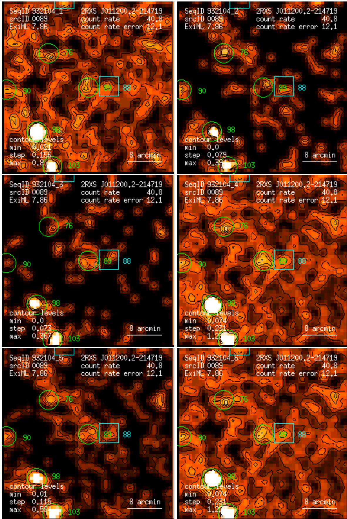
Figure 89: RASS 932104: detection 0089: band rate images, Gaussian filter: (1) PSPC channels 11 – 41, (2) 52 – 90, (3) 91 – 201, (4) 11 – 235, (5) 52 – 201, (6) 11 – 201. Broad band rates in counts/ks. Band rate contour levels in counts/ks/arcmin 2 .
