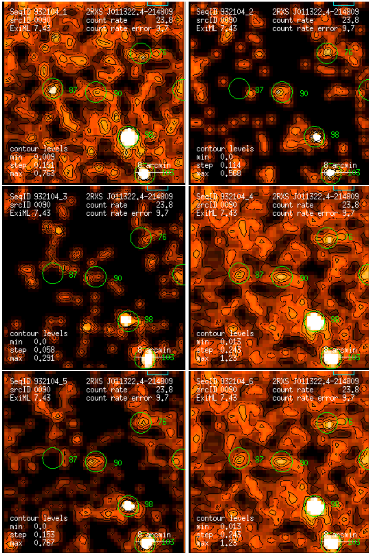
Figure 90: RASS 932104: detection 0090: band rate images, Gaussian filter: (1) PSPC channels 11 – 41, (2) 52 – 90, (3) 91 – 201, (4) 11 – 235, (5) 52 – 201, (6) 11 – 201. Broad band rates in counts/ks. Band rate contour levels in counts/ks/arcmin 2 .
