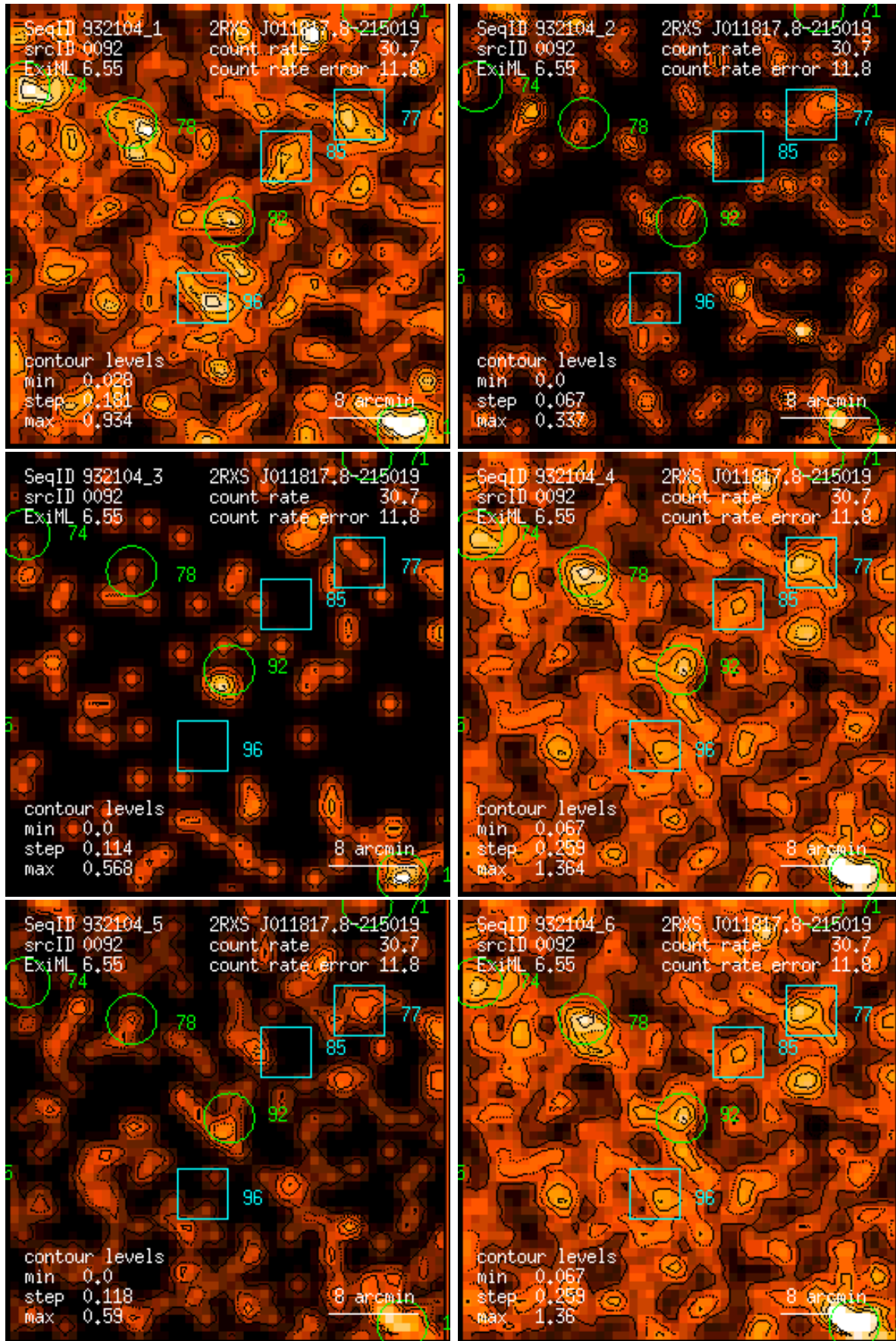
Figure 92: RASS 932104: detection 0092: band rate images, Gaussian filter: (1) PSPC channels 11 – 41, (2) 52 – 90, (3) 91 – 201, (4) 11 – 235, (5) 52 – 201, (6) 11 – 201. Broad band rates in counts/ks. Band rate contour levels in counts/ks/arcmin 2 .
