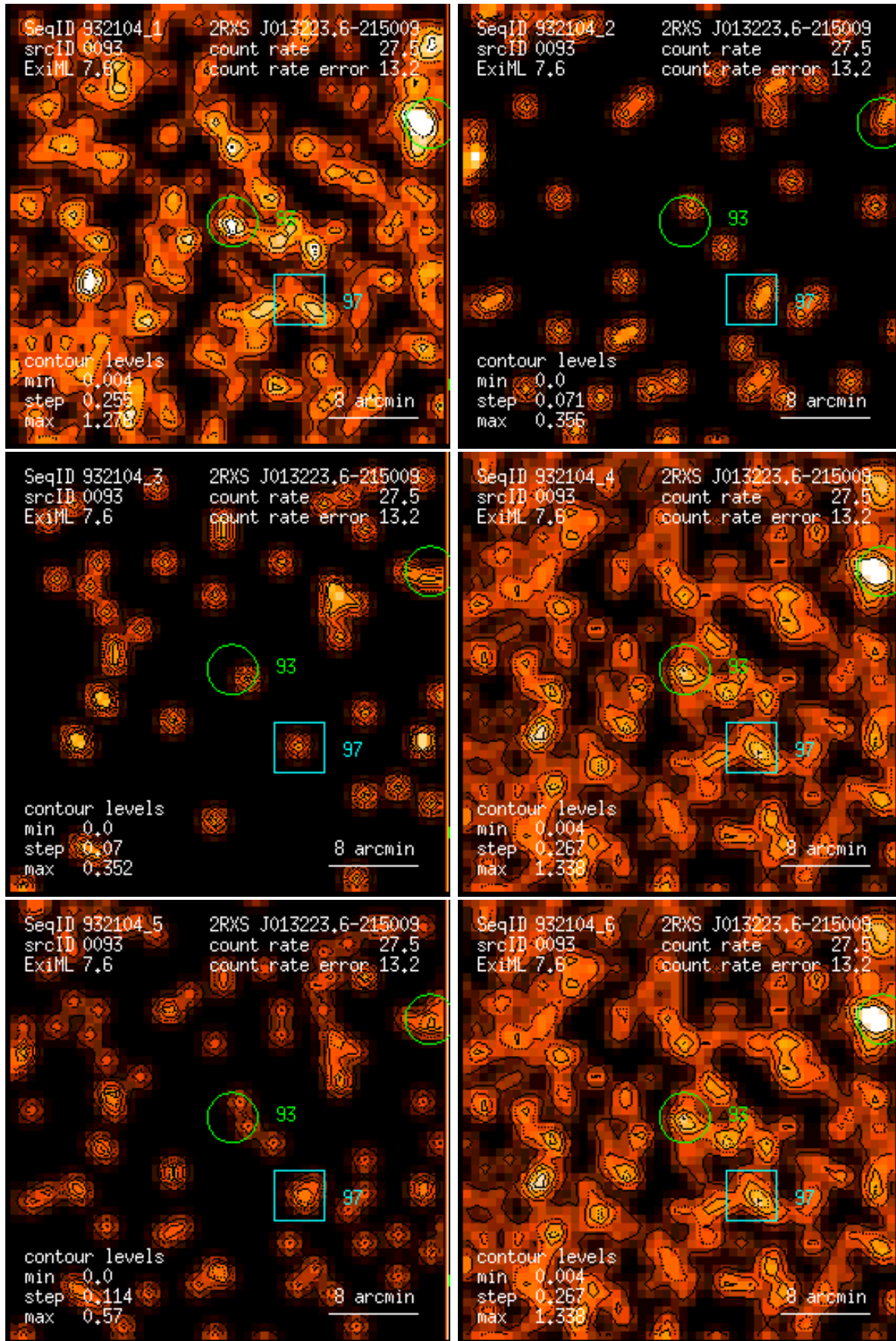
Figure 93: RASS 932104: detection 0093: band rate images, Gaussian filter: (1) PSPC channels 11 – 41, (2) 52 – 90, (3) 91 – 201, (4) 11 – 235, (5) 52 – 201, (6) 11 – 201. Broad band rates in counts/ks. Band rate contour levels in counts/ks/arcmin 2 .
