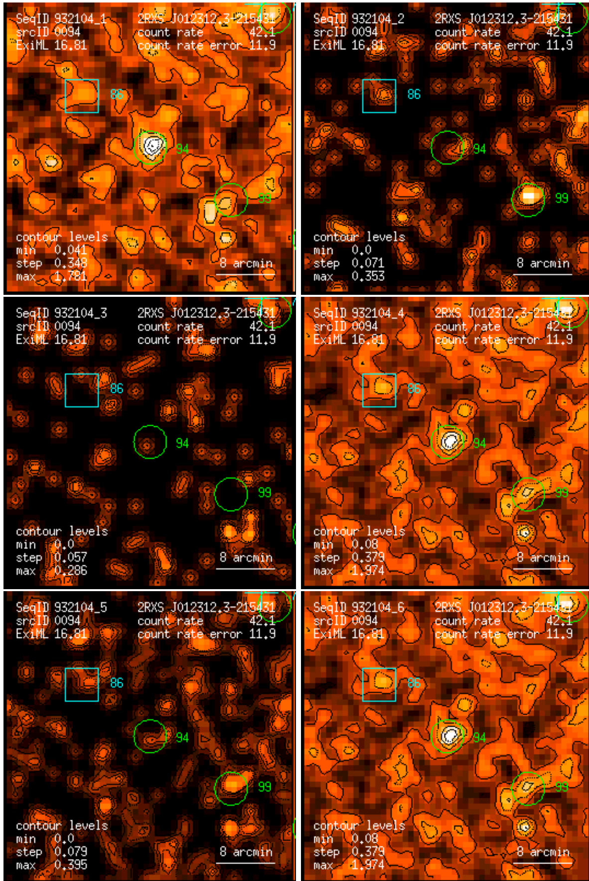
Figure 94: RASS 932104: detection 0094: band rate images, Gaussian filter: (1) PSPC channels 11 – 41, (2) 52 – 90, (3) 91 – 201, (4) 11 – 235, (5) 52 – 201, (6) 11 – 201. Broad band rates in counts/ks. Band rate contour levels in counts/ks/arcmin 2 .
