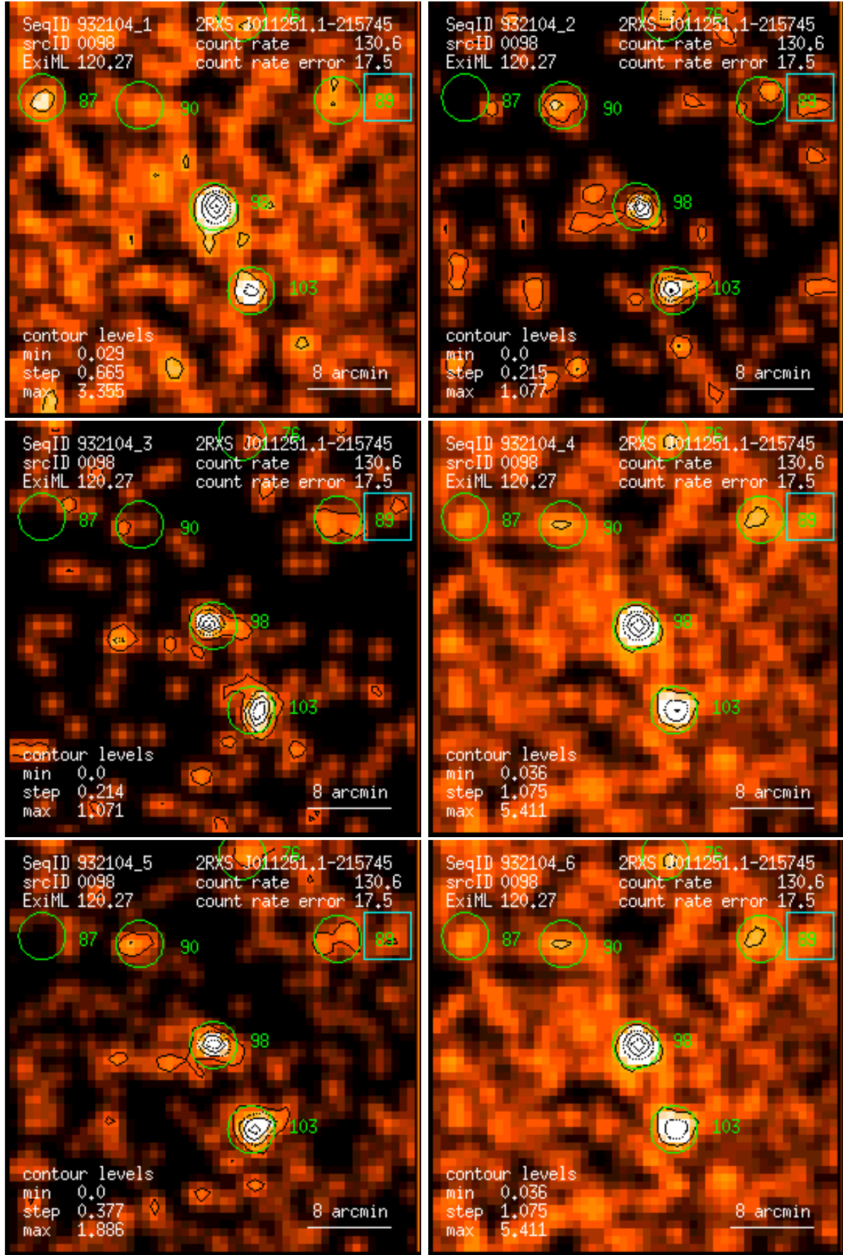
Figure 98: RASS 932104: detection 0098: band rate images, Gaussian filter: (1) PSPC channels 11 – 41, (2) 52 – 90, (3) 91 – 201, (4) 11 – 235, (5) 52 – 201, (6) 11 – 201. Broad band rates in counts/ks. Band rate contour levels in counts/ks/arcmin 2 .
