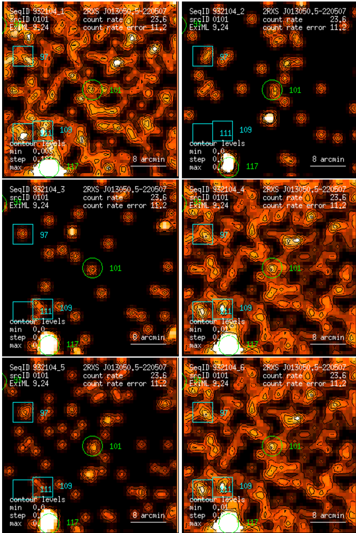
Figure 101: RASS 932104: detection 0101: band rate images, Gaussian filter: (1) PSPC channels 11 – 41, (2) 52 – 90, (3) 91 – 201, (4) 11 – 235, (5) 52 – 201, (6) 11 – 201. Broad band rates in counts/ks. Band rate contour levels in counts/ks/arcmin 2 .
