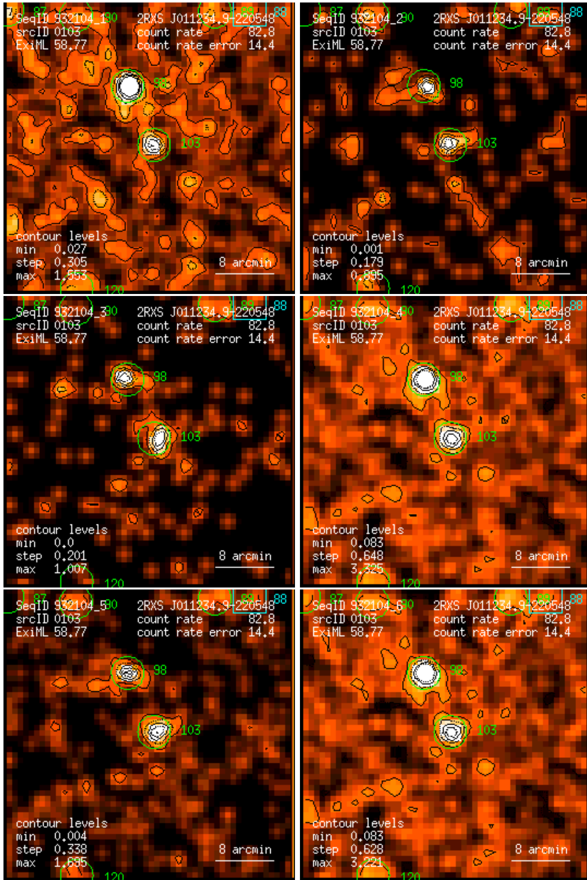
Figure 103: RASS 932104: detection 0103: band rate images, Gaussian filter: (1) PSPC channels 11 – 41, (2) 52 – 90, (3) 91 – 201, (4) 11 – 235, (5) 52 – 201, (6) 11 – 201. Broad band rates in counts/ks. Band rate contour levels in counts/ks/arcmin 2 .
