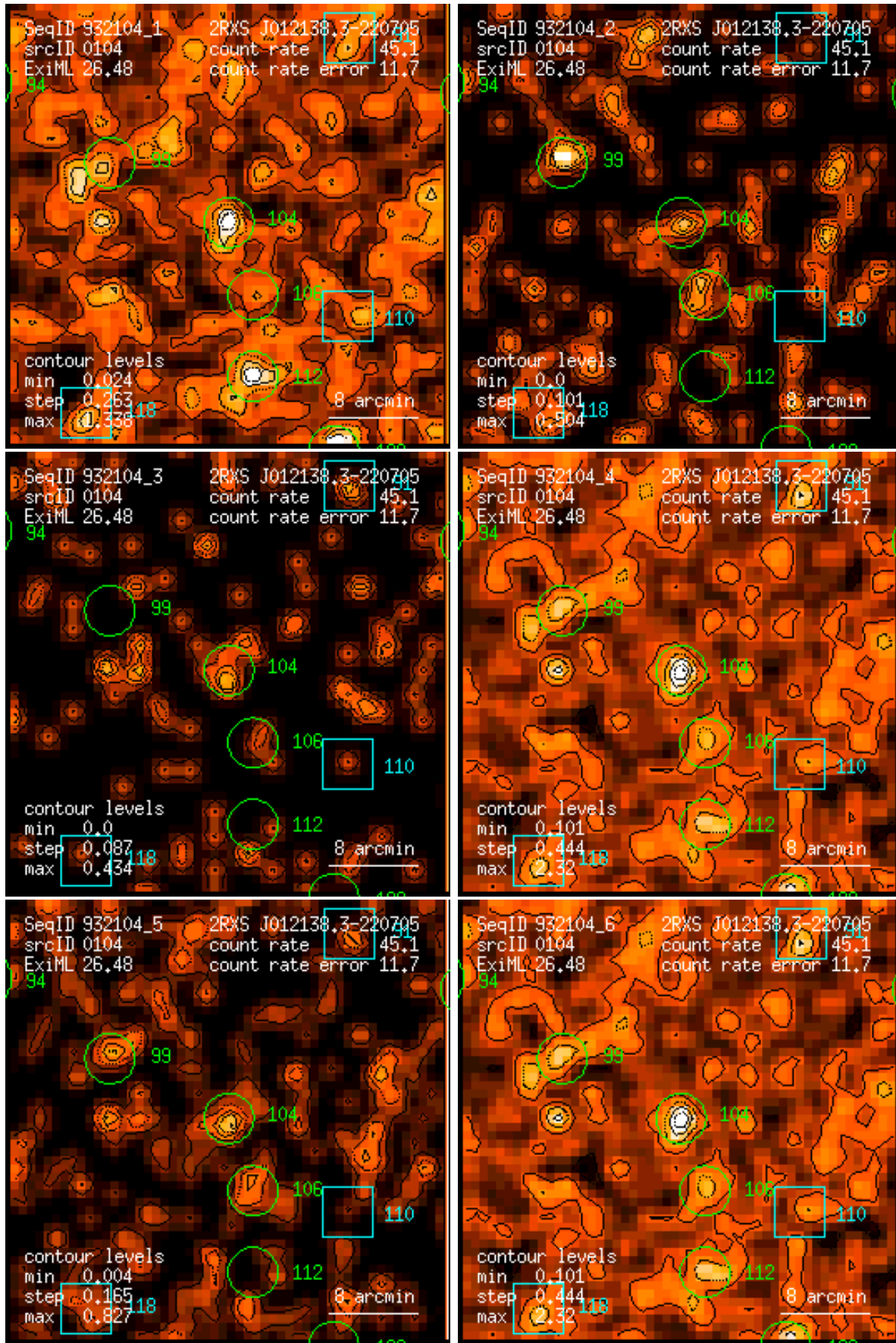
Figure 104: RASS 932104: detection 0104: band rate images, Gaussian filter: (1) PSPC channels 11 – 41, (2) 52 – 90, (3) 91 – 201, (4) 11 – 235, (5) 52 – 201, (6) 11 – 201. Broad band rates in counts/ks. Band rate contour levels in counts/ks/arcmin 2 .
