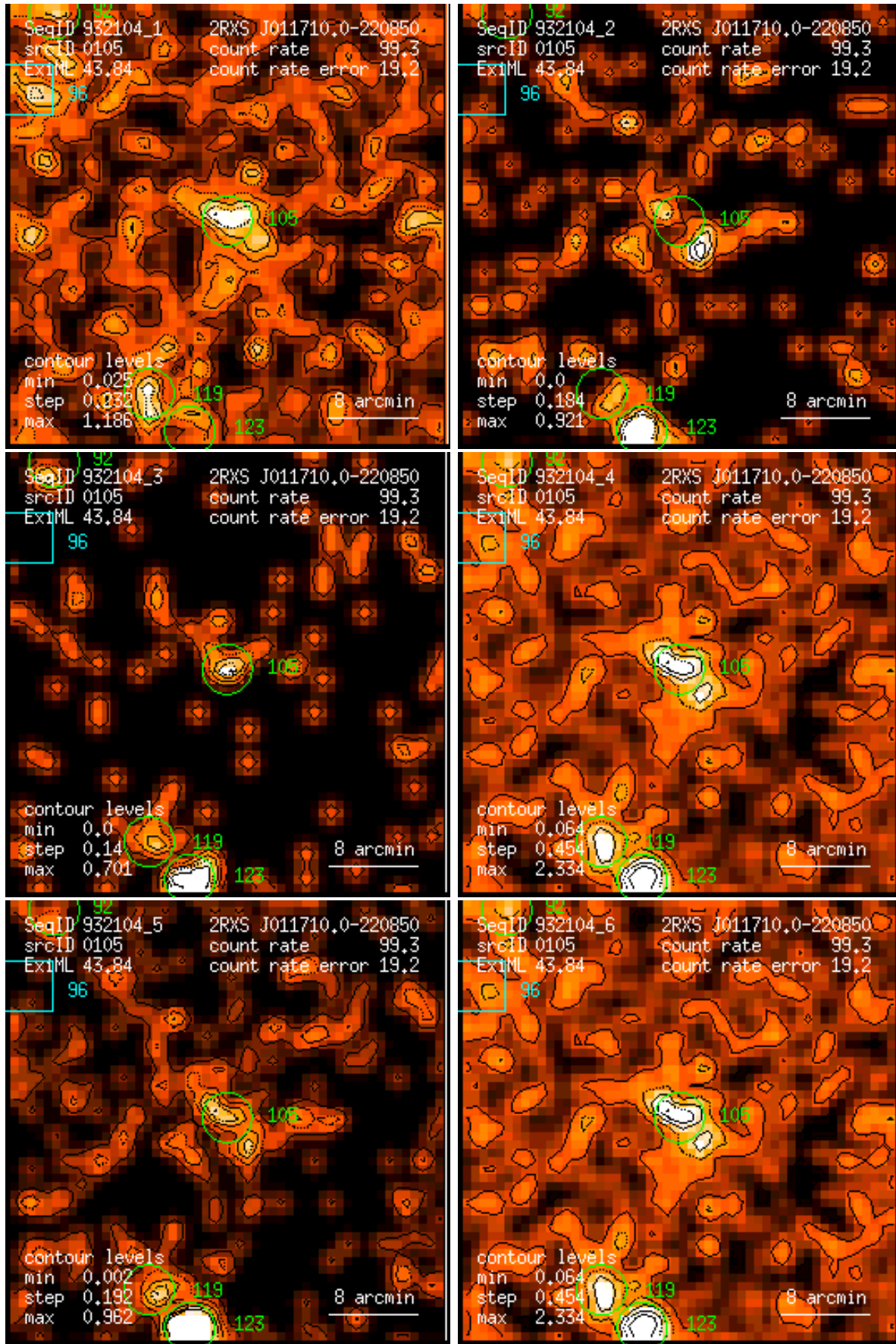
Figure 105: RASS 932104: detection 0105: band rate images, Gaussian filter: (1) PSPC channels 11 – 41, (2) 52 – 90, (3) 91 – 201, (4) 11 – 235, (5) 52 – 201, (6) 11 – 201. Broad band rates in counts/ks. Band rate contour levels in counts/ks/arcmin 2 .
