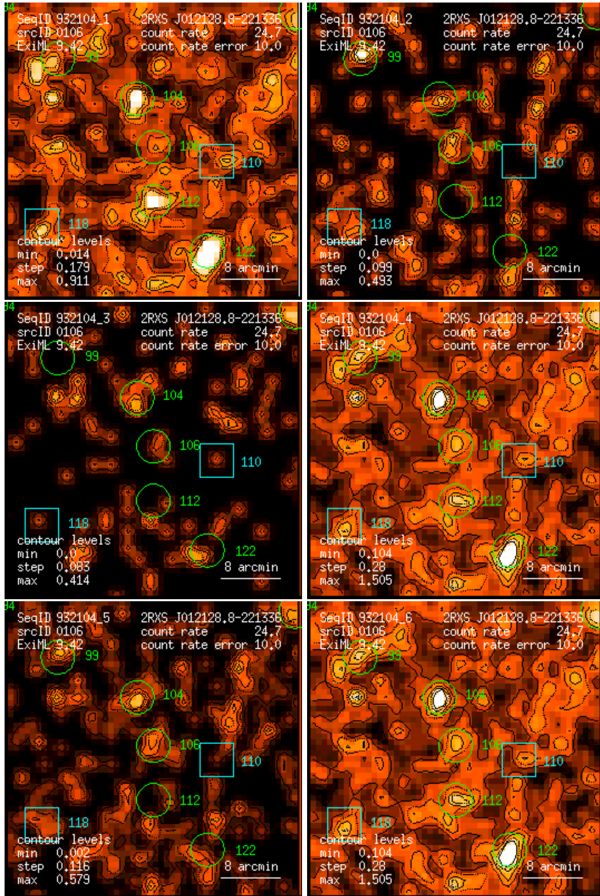
Figure 106: RASS 932104: detection 0106: band rate images, Gaussian filter: (1) PSPC channels 11 – 41, (2) 52 – 90, (3) 91 – 201, (4) 11 – 235, (5) 52 – 201, (6) 11 – 201. Broad band rates in counts/ks. Band rate contour levels in counts/ks/arcmin 2 .
