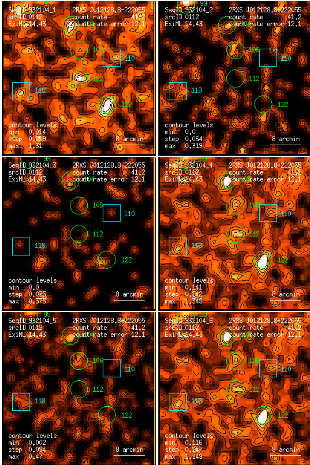
Figure 112: RASS 932104: detection 0112: band rate images, Gaussian filter: (1) PSPC channels 11 – 41, (2) 52 – 90, (3) 91 – 201, (4) 11 – 235, (5) 52 – 201, (6) 11 – 201. Broad band rates in counts/ks. Band rate contour levels in counts/ks/arcmin 2 .
