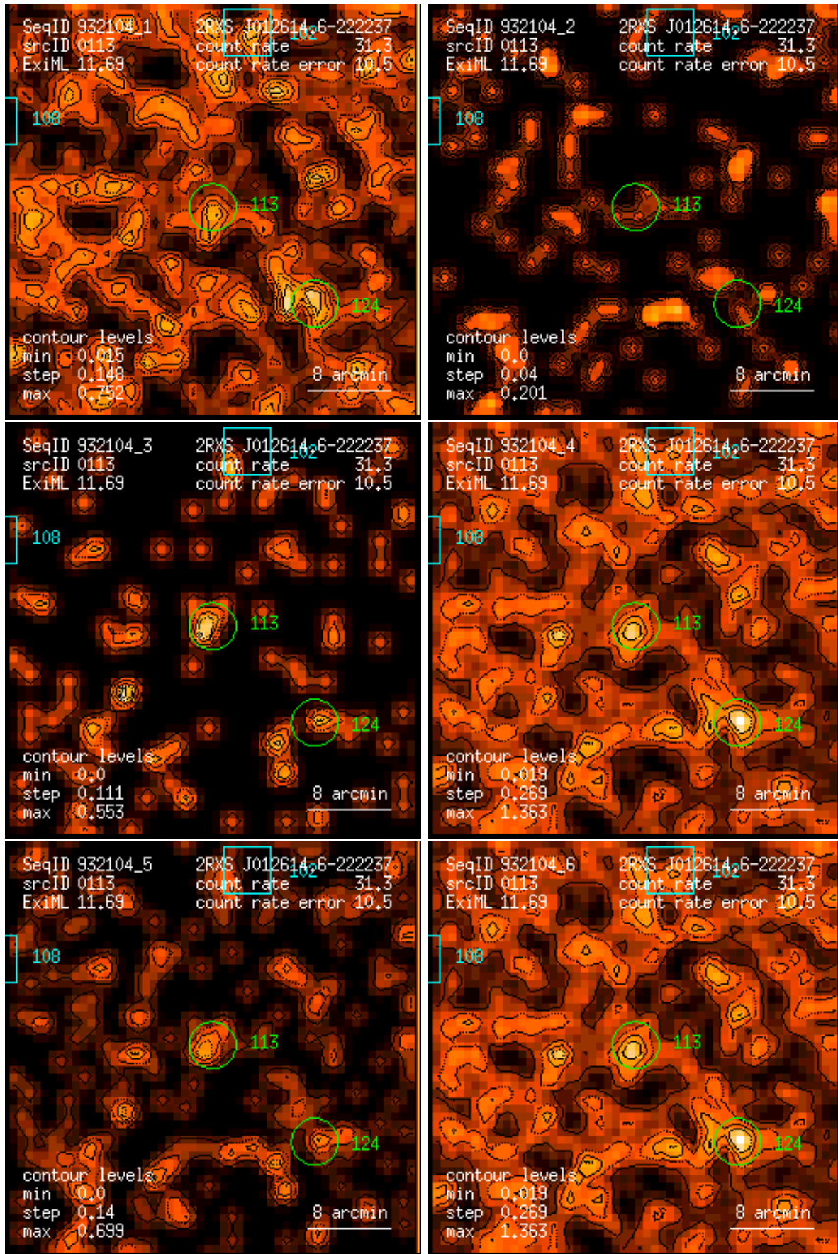
Figure 113: RASS 932104: detection 0113: band rate images, Gaussian filter: (1) PSPC channels 11 – 41, (2) 52 – 90, (3) 91 – 201, (4) 11 – 235, (5) 52 – 201, (6) 11 – 201. Broad band rates in counts/ks. Band rate contour levels in counts/ks/arcmin 2 .
