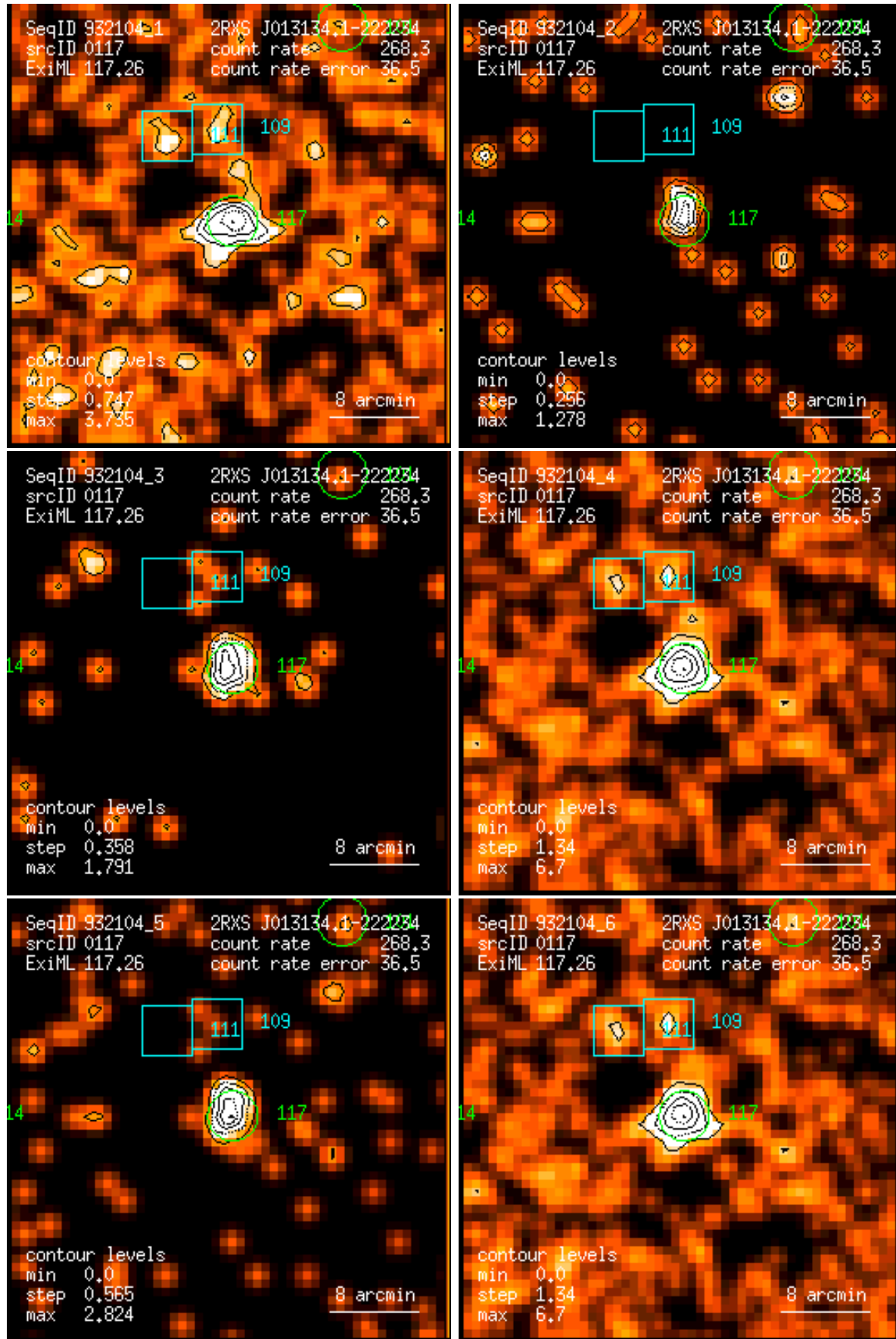
Figure 117: RASS 932104: detection 0117: band rate images, Gaussian filter: (1) PSPC channels 11 – 41, (2) 52 – 90, (3) 91 – 201, (4) 11 – 235, (5) 52 – 201, (6) 11 – 201. Broad band rates in counts/ks. Band rate contour levels in counts/ks/arcmin 2 .
