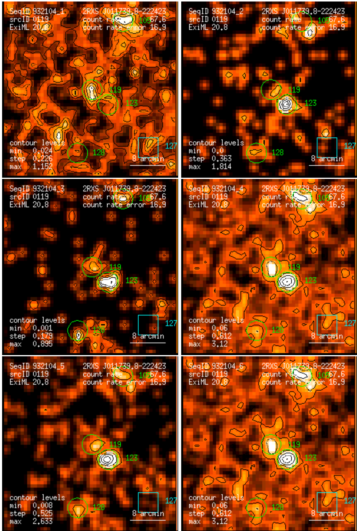
Figure 119: RASS 932104: detection 0119: band rate images, Gaussian filter: (1) PSPC channels 11 – 41, (2) 52 – 90, (3) 91 – 201, (4) 11 – 235, (5) 52 – 201, (6) 11 – 201. Broad band rates in counts/ks. Band rate contour levels in counts/ks/arcmin 2 .
