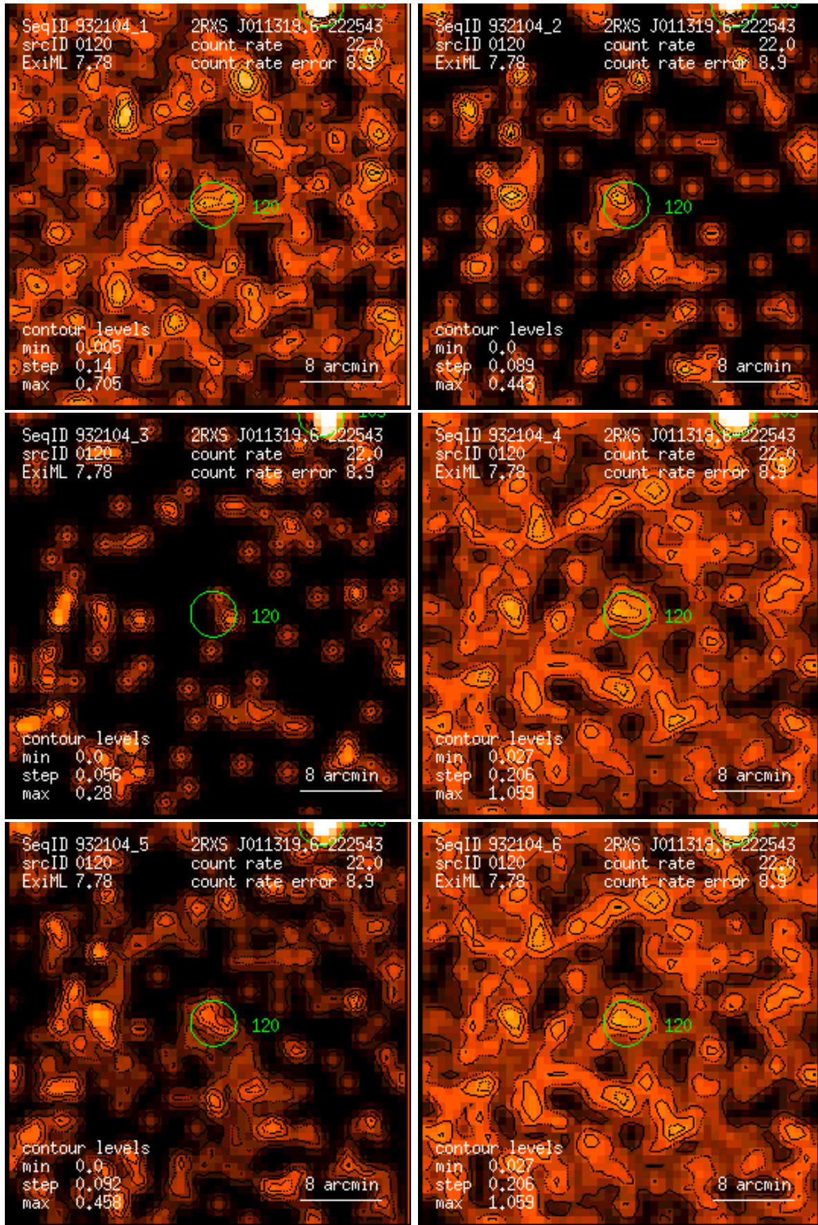
Figure 120: RASS 932104: detection 0120: band rate images, Gaussian filter: (1) PSPC channels 11 – 41, (2) 52 – 90, (3) 91 – 201, (4) 11 – 235, (5) 52 – 201, (6) 11 – 201. Broad band rates in counts/ks. Band rate contour levels in counts/ks/arcmin 2 .
