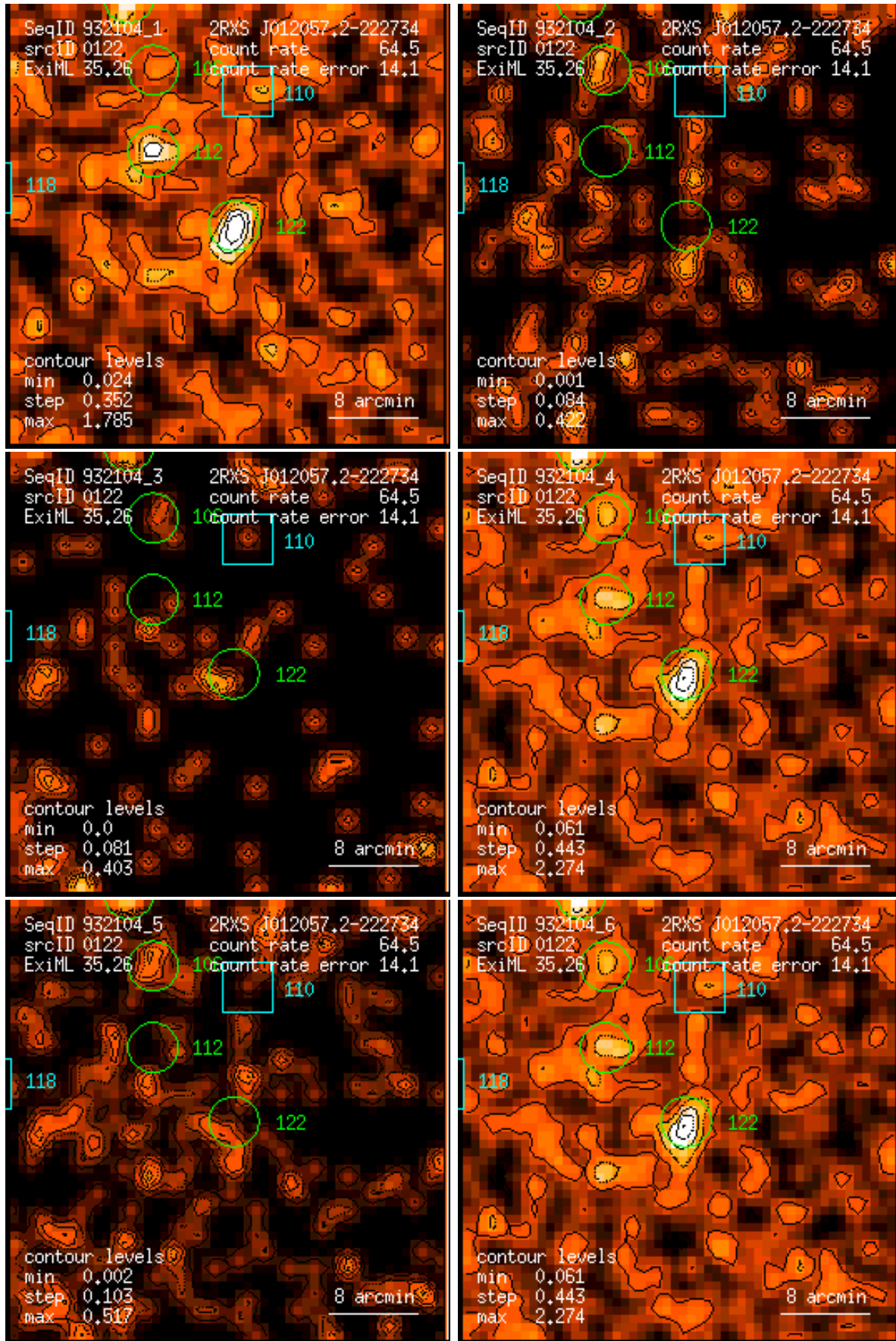
Figure 122: RASS 932104: detection 0122: band rate images, Gaussian filter: (1) PSPC channels 11 – 41, (2) 52 – 90, (3) 91 – 201, (4) 11 – 235, (5) 52 – 201, (6) 11 – 201. Broad band rates in counts/ks. Band rate contour levels in counts/ks/arcmin 2 .
