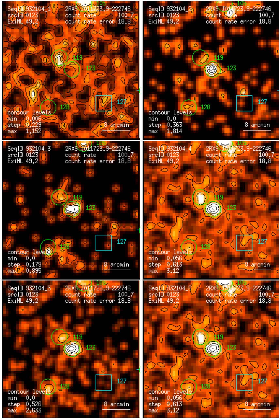
Figure 123: RASS 932104: detection 0123: band rate images, Gaussian filter: (1) PSPC channels 11 – 41, (2) 52 – 90, (3) 91 – 201, (4) 11 – 235, (5) 52 – 201, (6) 11 – 201. Broad band rates in counts/ks. Band rate contour levels in counts/ks/arcmin 2 .
