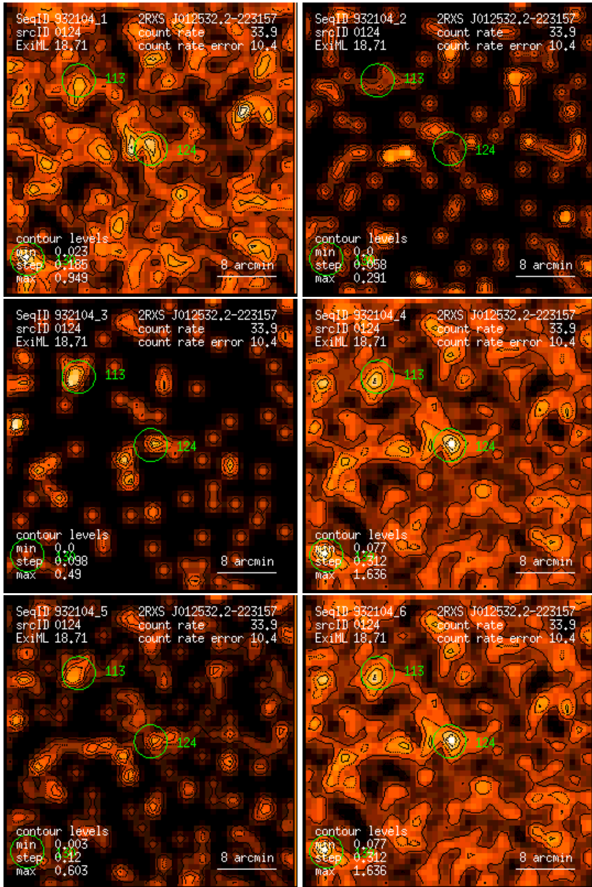
Figure 124: RASS 932104: detection 0124: band rate images, Gaussian filter: (1) PSPC channels 11 – 41, (2) 52 – 90, (3) 91 – 201, (4) 11 – 235, (5) 52 – 201, (6) 11 – 201. Broad band rates in counts/ks. Band rate contour levels in counts/ks/arcmin 2 .
