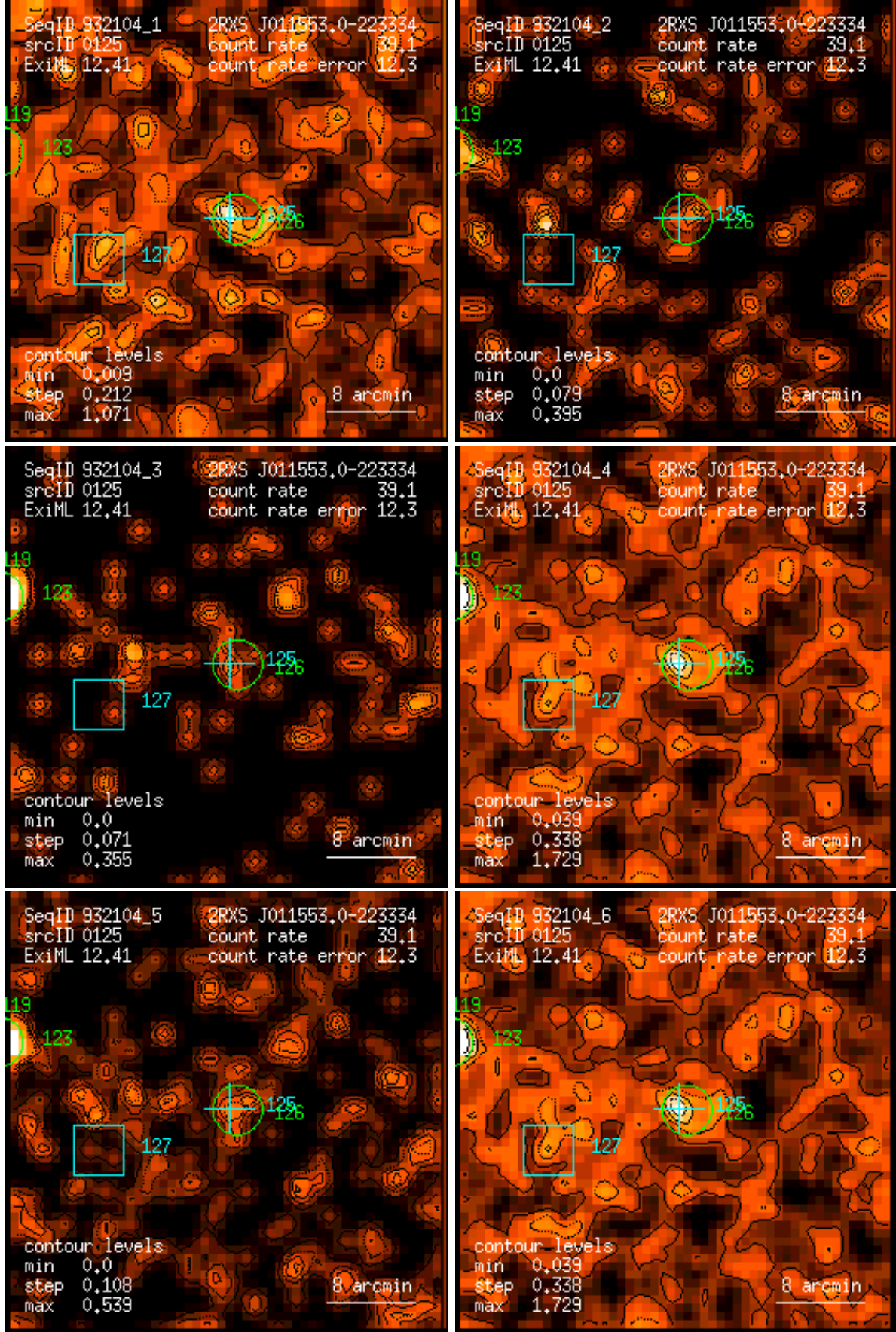
Figure 125: RASS 932104: detection 0125: band rate images, Gaussian filter: (1) PSPC channels 11 – 41, (2) 52 – 90, (3) 91 – 201, (4) 11 – 235, (5) 52 – 201, (6) 11 – 201. Broad band rates in counts/ks. Band rate contour levels in counts/ks/arcmin 2 .
