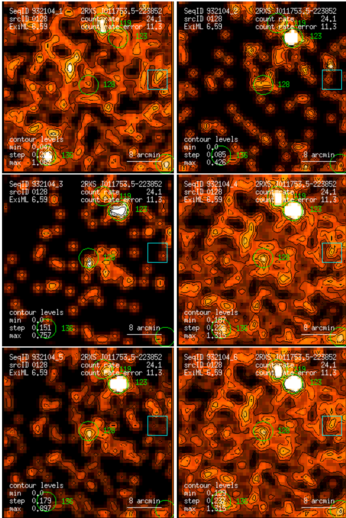
Figure 128: RASS 932104: detection 0128: band rate images, Gaussian filter: (1) PSPC channels 11 – 41, (2) 52 – 90, (3) 91 – 201, (4) 11 – 235, (5) 52 – 201, (6) 11 – 201. Broad band rates in counts/ks. Band rate contour levels in counts/ks/arcmin 2 .
