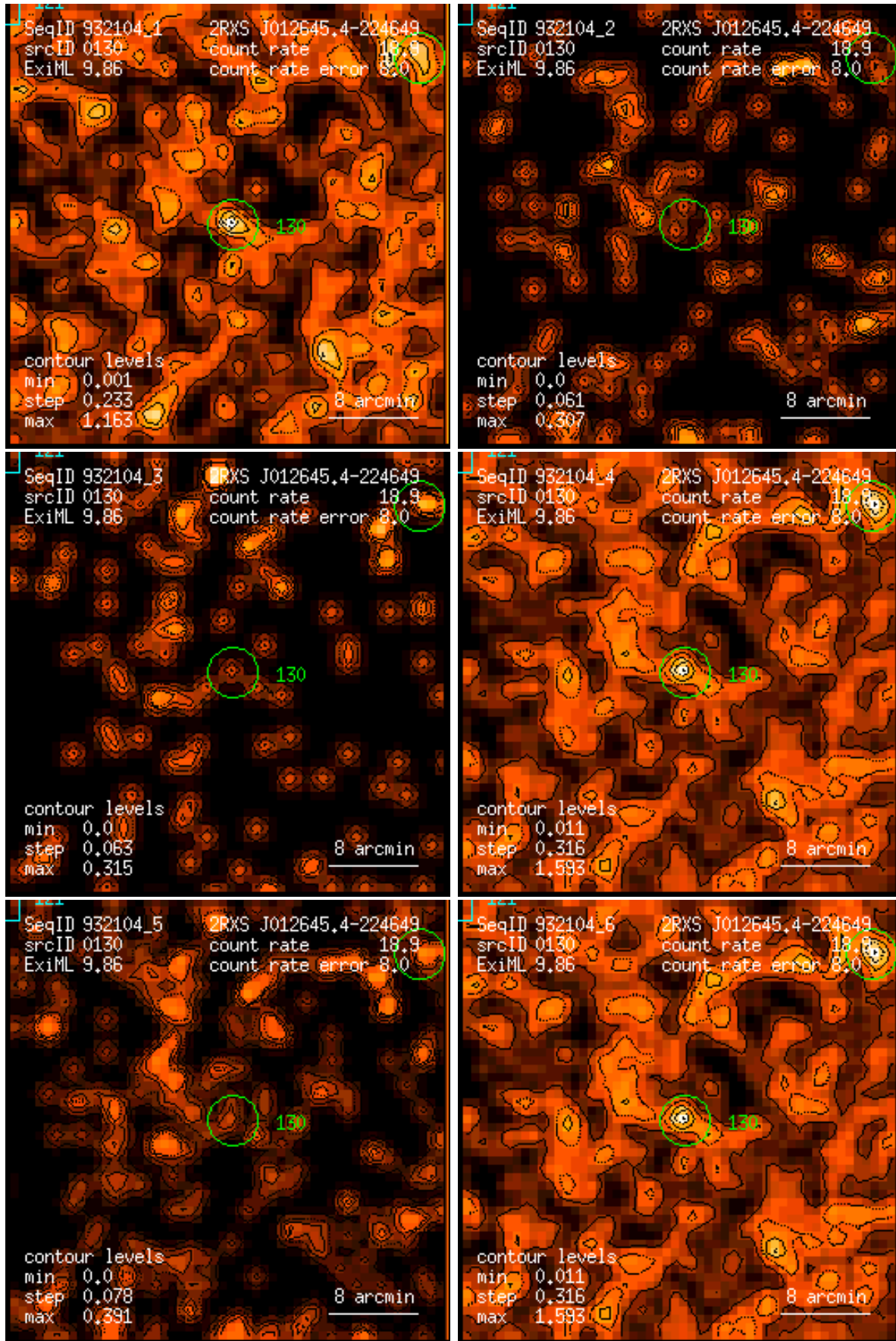
Figure 130: RASS 932104: detection 0130: band rate images, Gaussian filter: (1) PSPC channels 11 – 41, (2) 52 – 90, (3) 91 – 201, (4) 11 – 235, (5) 52 – 201, (6) 11 – 201. Broad band rates in counts/ks. Band rate contour levels in counts/ks/arcmin 2 .
