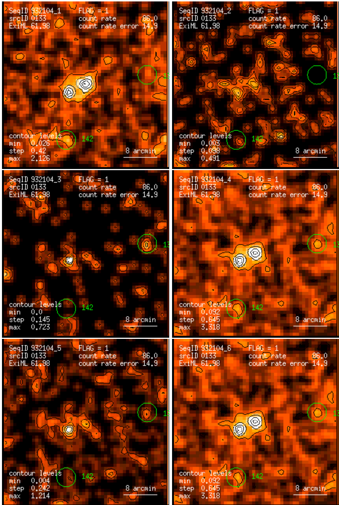
Figure 133: RASS 932104: detection 0133: band rate images, Gaussian filter: (1) PSPC channels 11 – 41, (2) 52 – 90, (3) 91 – 201, (4) 11 – 235, (5) 52 – 201, (6) 11 – 201. Broad band rates in counts/ks. Band rate contour levels in counts/ks/arcmin 2 .
