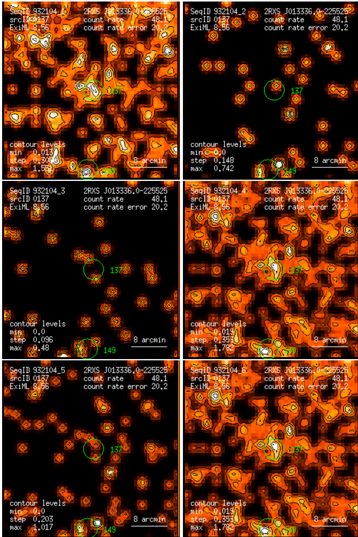
Figure 137: RASS 932104: detection 0137: band rate images, Gaussian filter: (1) PSPC channels 11 – 41, (2) 52 – 90, (3) 91 – 201, (4) 11 – 235, (5) 52 – 201, (6) 11 – 201. Broad band rates in counts/ks. Band rate contour levels in counts/ks/arcmin 2 .
