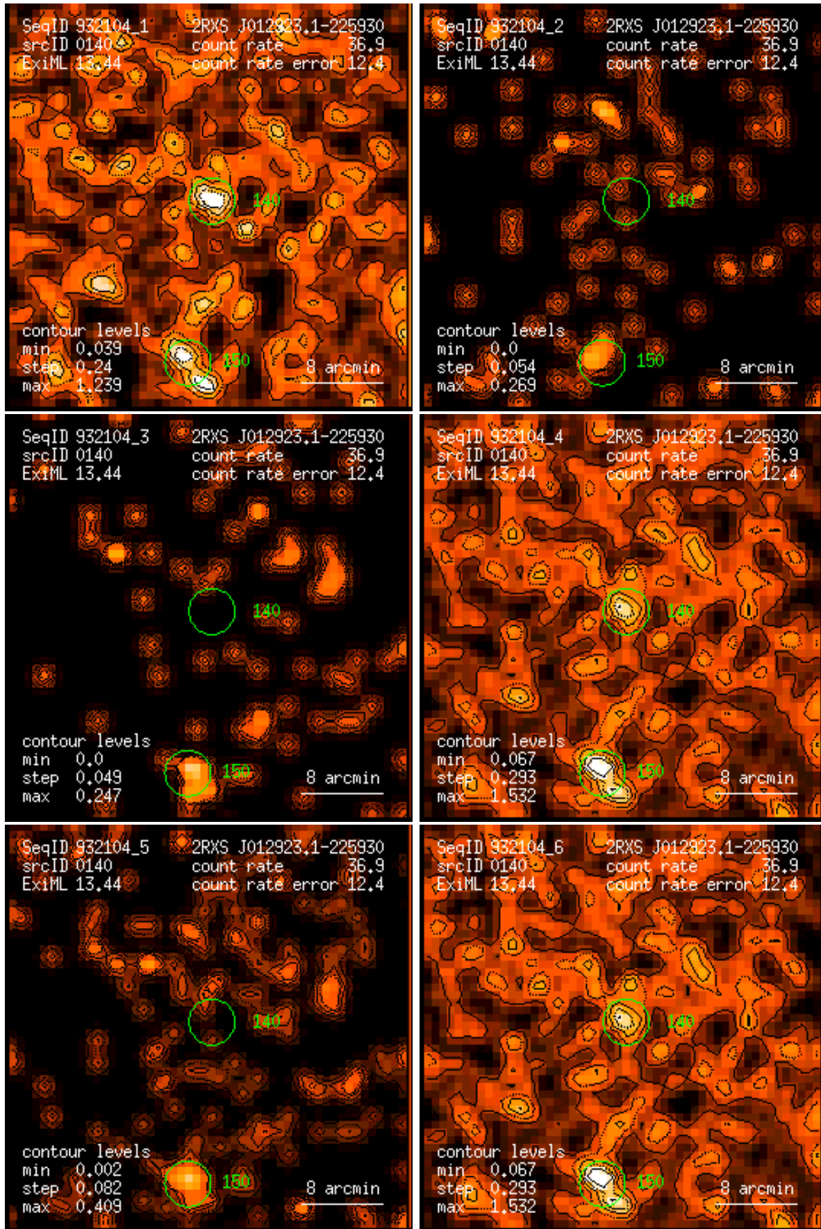
Figure 140: RASS 932104: detection 0140: band rate images, Gaussian filter: (1) PSPC channels 11 – 41, (2) 52 – 90, (3) 91 – 201, (4) 11 – 235, (5) 52 – 201, (6) 11 – 201. Broad band rates in counts/ks. Band rate contour levels in counts/ks/arcmin 2 .
