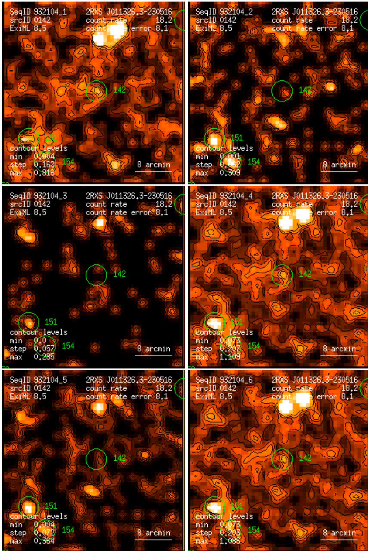
Figure 142: RASS 932104: detection 0142: band rate images, Gaussian filter: (1) PSPC channels 11 – 41, (2) 52 – 90, (3) 91 – 201, (4) 11 – 235, (5) 52 – 201, (6) 11 – 201. Broad band rates in counts/ks. Band rate contour levels in counts/ks/arcmin 2 .
