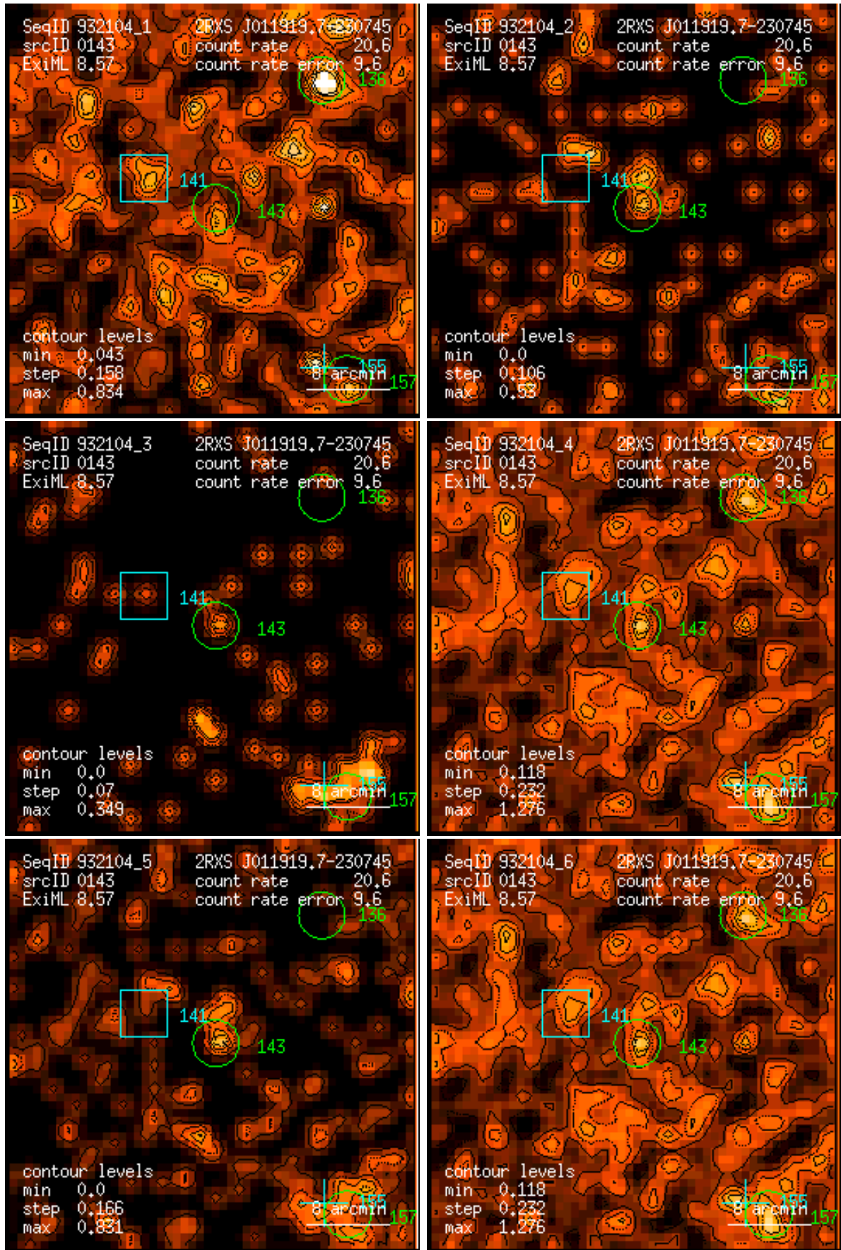
Figure 143: RASS 932104: detection 0143: band rate images, Gaussian filter: (1) PSPC channels 11 – 41, (2) 52 – 90, (3) 91 – 201, (4) 11 – 235, (5) 52 – 201, (6) 11 – 201. Broad band rates in counts/ks. Band rate contour levels in counts/ks/arcmin 2 .
