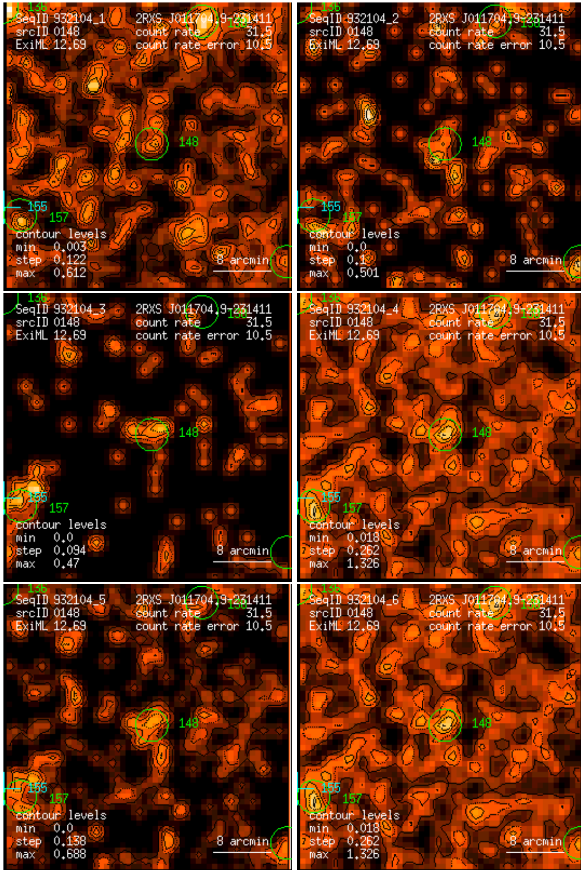
Figure 148: RASS 932104: detection 0148: band rate images, Gaussian filter: (1) PSPC channels 11 – 41, (2) 52 – 90, (3) 91 – 201, (4) 11 – 235, (5) 52 – 201, (6) 11 – 201. Broad band rates in counts/ks. Band rate contour levels in counts/ks/arcmin 2 .
