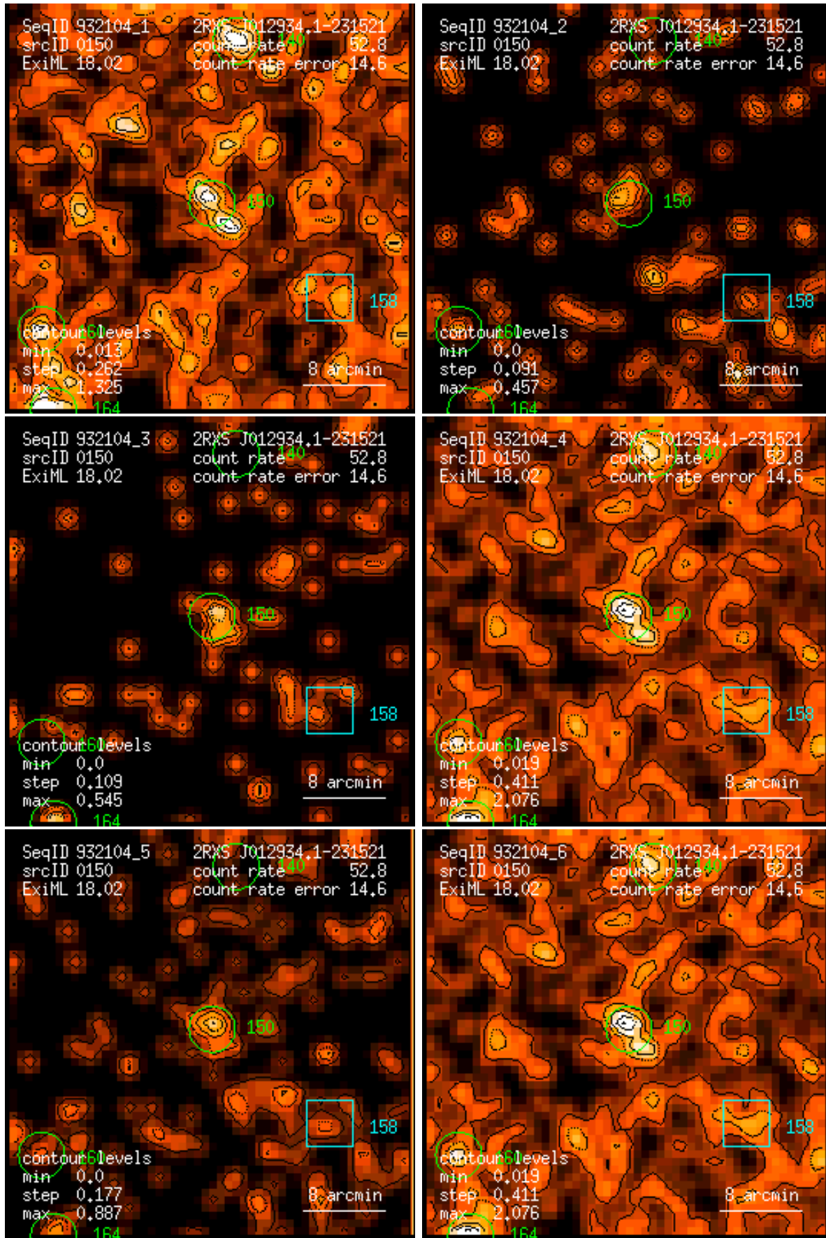
Figure 150: RASS 932104: detection 0150: band rate images, Gaussian filter: (1) PSPC channels 11 – 41, (2) 52 – 90, (3) 91 – 201, (4) 11 – 235, (5) 52 – 201, (6) 11 – 201. Broad band rates in counts/ks. Band rate contour levels in counts/ks/arcmin 2 .
