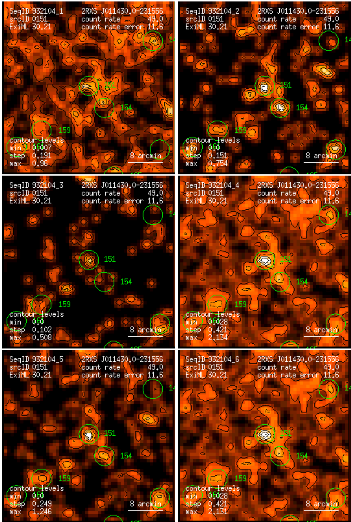
Figure 151: RASS 932104: detection 0151: band rate images, Gaussian filter: (1) PSPC channels 11 – 41, (2) 52 – 90, (3) 91 – 201, (4) 11 – 235, (5) 52 – 201, (6) 11 – 201. Broad band rates in counts/ks. Band rate contour levels in counts/ks/arcmin 2 .
