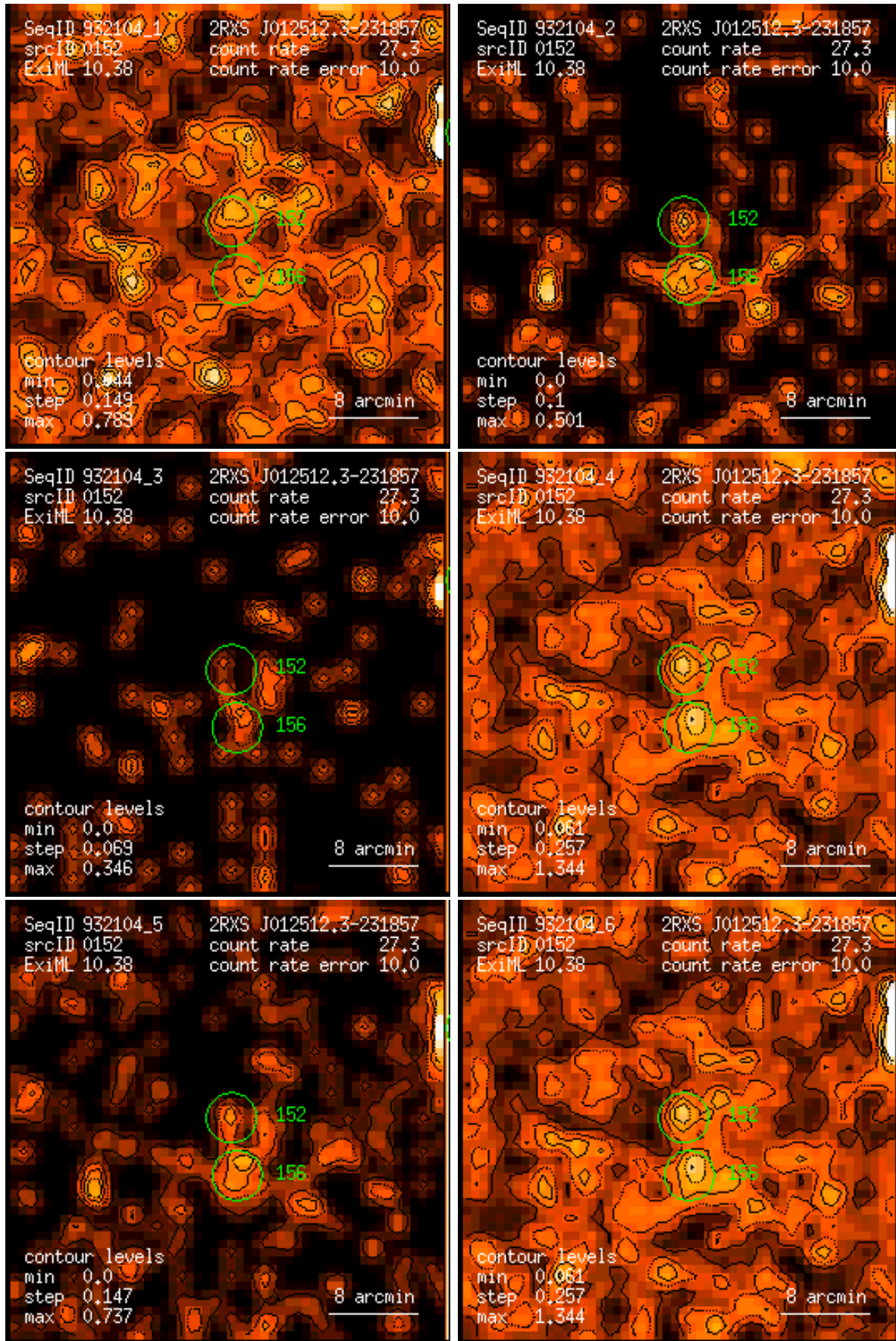
Figure 152: RASS 932104: detection 0152: band rate images, Gaussian filter: (1) PSPC channels 11 – 41, (2) 52 – 90, (3) 91 – 201, (4) 11 – 235, (5) 52 – 201, (6) 11 – 201. Broad band rates in counts/ks. Band rate contour levels in counts/ks/arcmin 2 .
