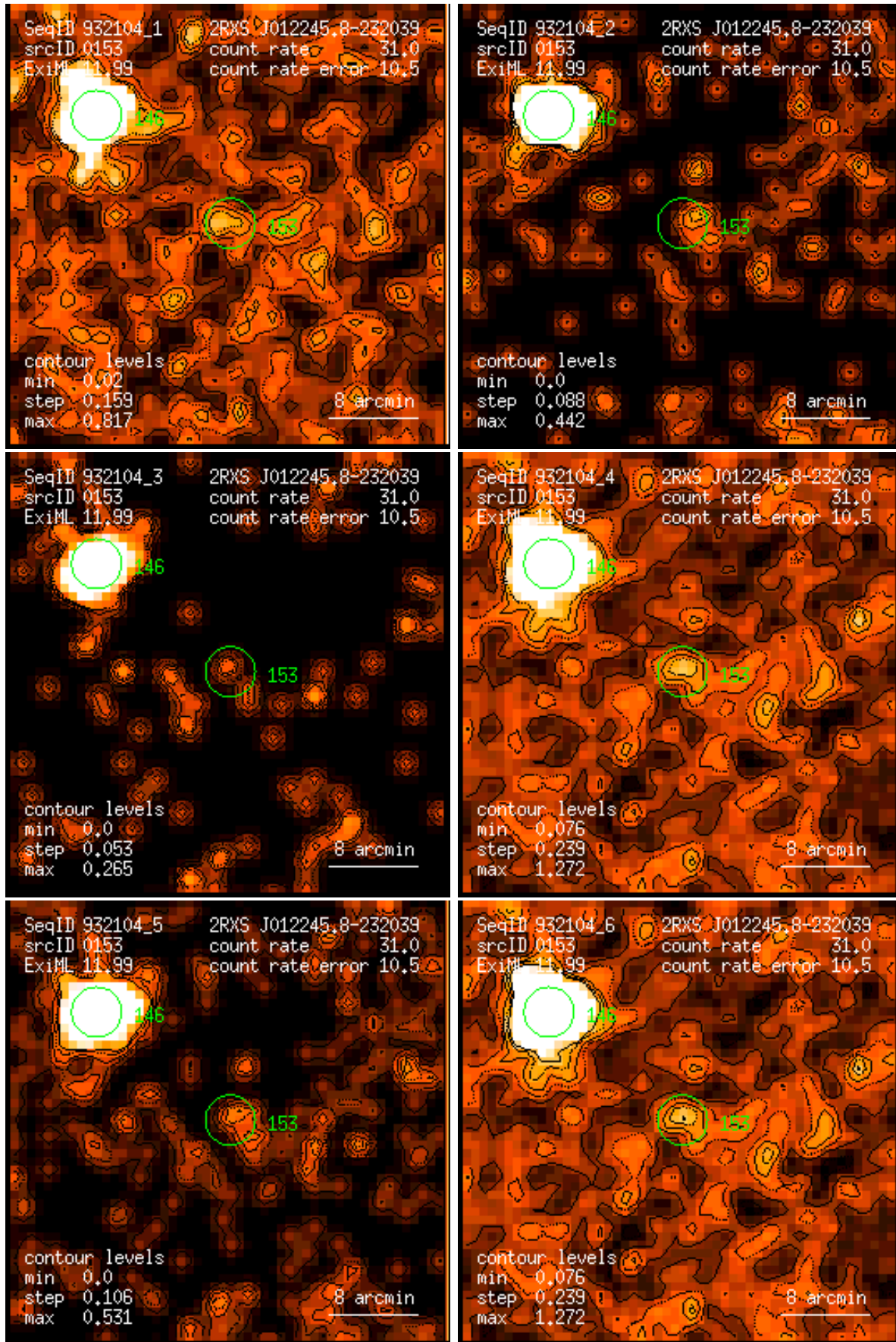
Figure 153: RASS 932104: detection 0153: band rate images, Gaussian filter: (1) PSPC channels 11 – 41, (2) 52 – 90, (3) 91 – 201, (4) 11 – 235, (5) 52 – 201, (6) 11 – 201. Broad band rates in counts/ks. Band rate contour levels in counts/ks/arcmin 2 .
