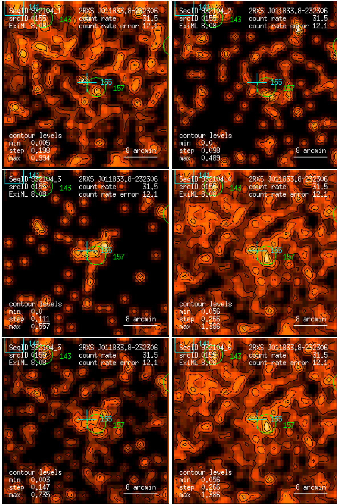
Figure 155: RASS 932104: detection 0155: band rate images, Gaussian filter: (1) PSPC channels 11 – 41, (2) 52 – 90, (3) 91 – 201, (4) 11 – 235, (5) 52 – 201, (6) 11 – 201. Broad band rates in counts/ks. Band rate contour levels in counts/ks/arcmin 2 .
