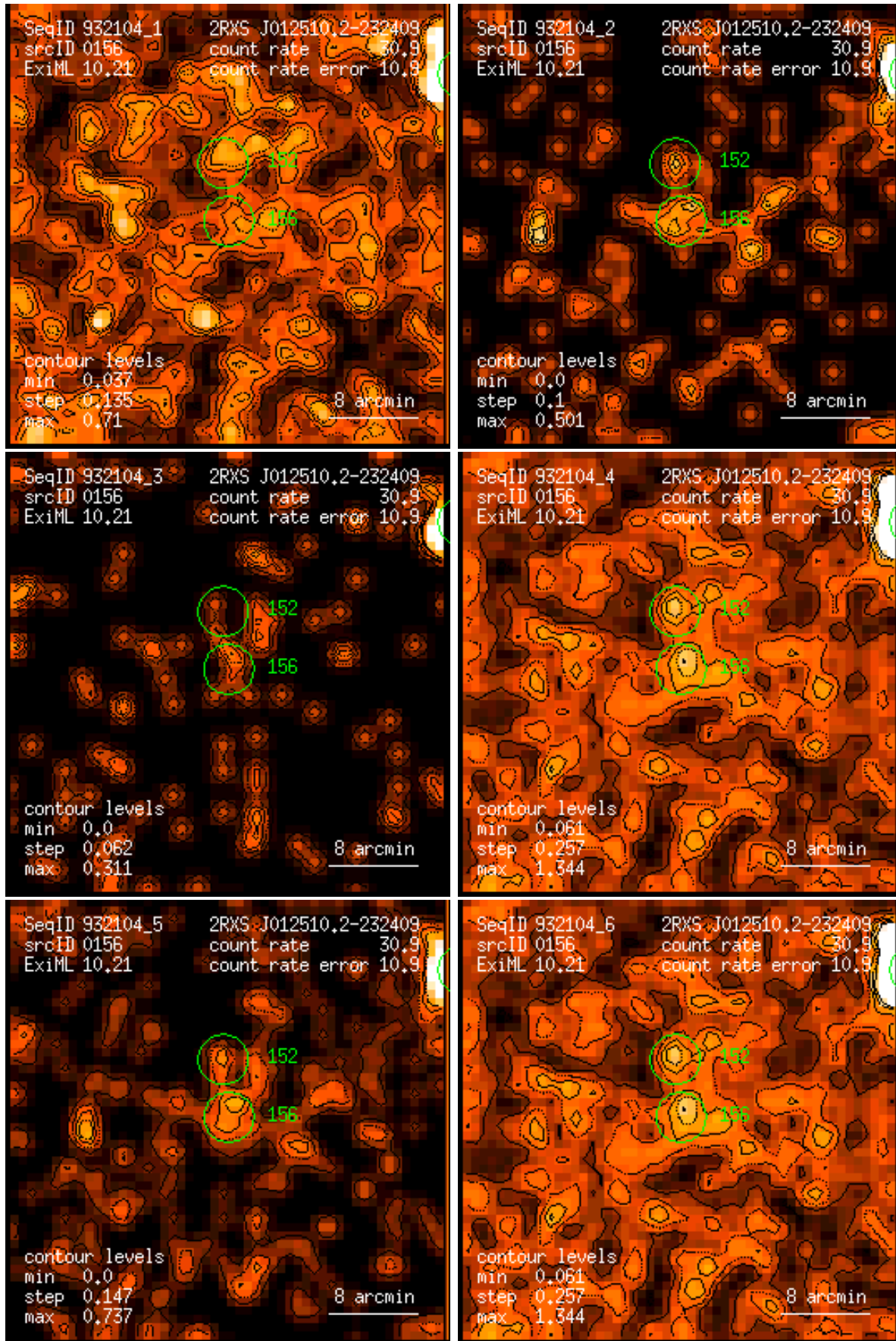
Figure 156: RASS 932104: detection 0156: band rate images, Gaussian filter: (1) PSPC channels 11 – 41, (2) 52 – 90, (3) 91 – 201, (4) 11 – 235, (5) 52 – 201, (6) 11 – 201. Broad band rates in counts/ks. Band rate contour levels in counts/ks/arcmin 2 .
